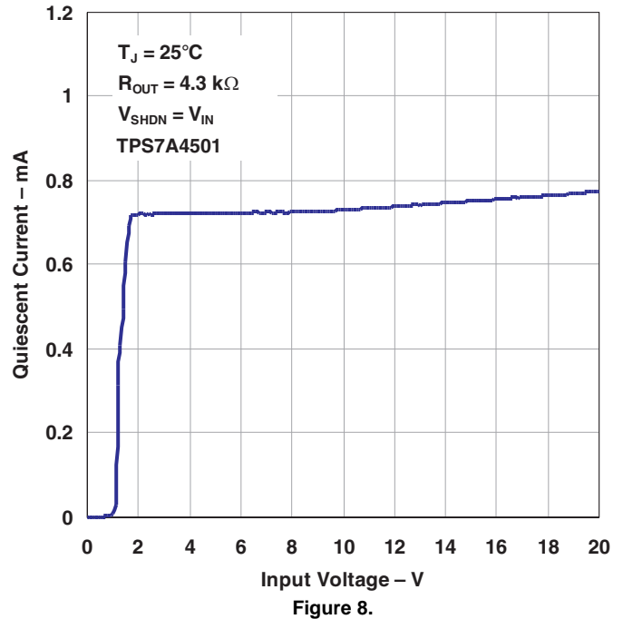
QUIESCENT CURRENT VS INPUT VOLTAGE
