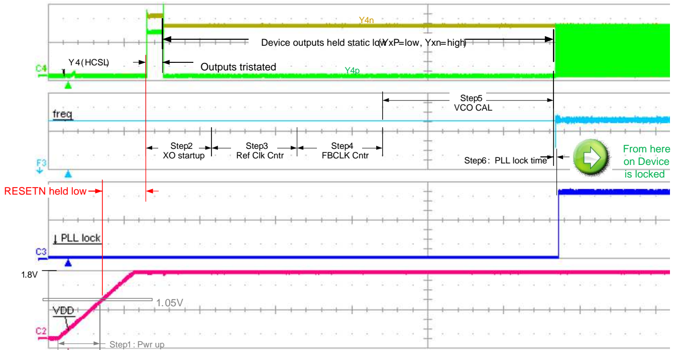
Figure 29. Power up Time
