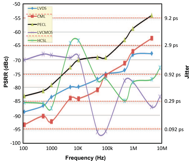
Figure 8. PSRR (in dBc and DJ [ps]) Over Frequency [Hz] and Output Signal Format ( f_{OUT} = 122\text{ MHz} )
