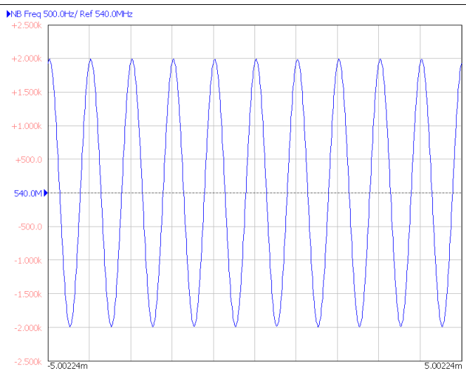
Figure 85. Simulated FM Modulation (20 times over-sampling)
