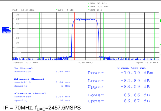
Figure 43. Single Carrier W-CDMA Test Mode 1
