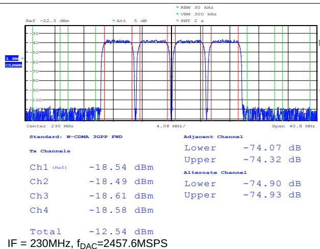
Figure 48. Four Carrier W-CDMA Test Mode 1
