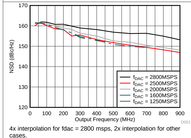
Figure 23. NSD vs Output Frequency Over f_{\text{DAC}}
