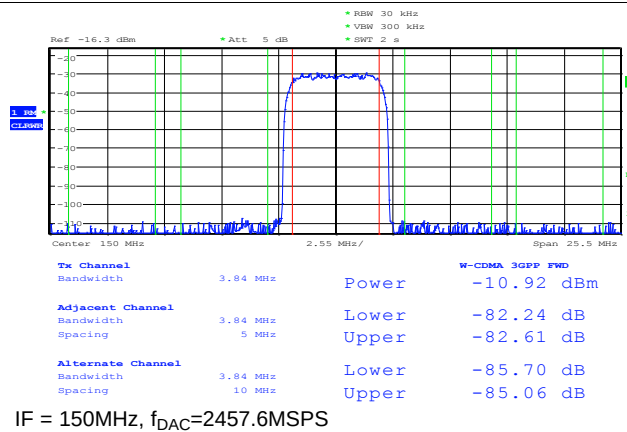
Figure 44. Single Carrier W-CDMA Test Mode 1
