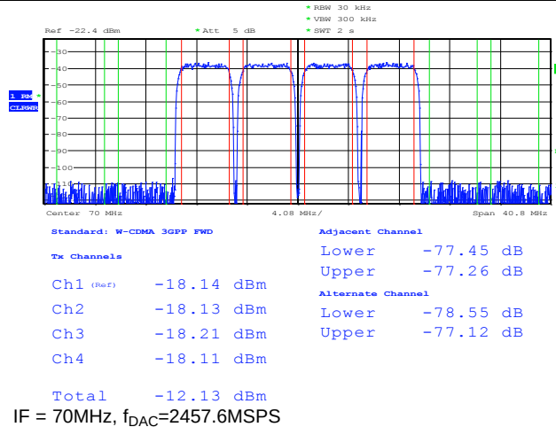
Figure 46. Four Carrier W-CDMA Test Mode 1
