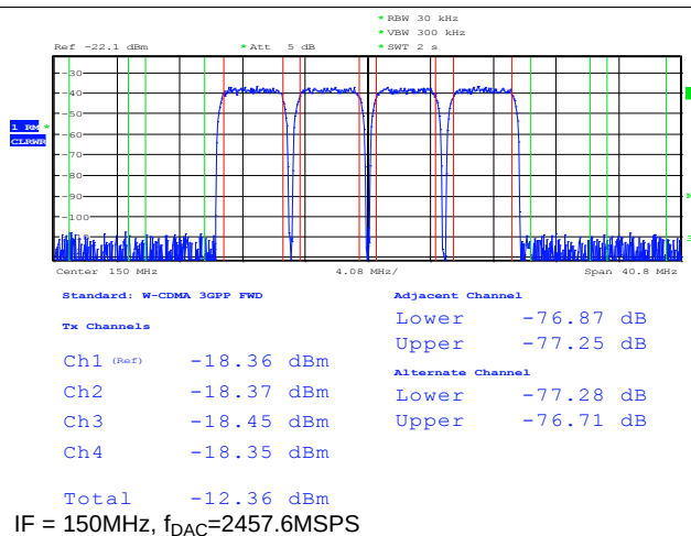
Figure 47. Four Carrier W-CDMA Test Mode 1
