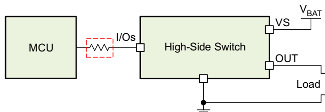
Figure 37. MCU I/O External Protection
