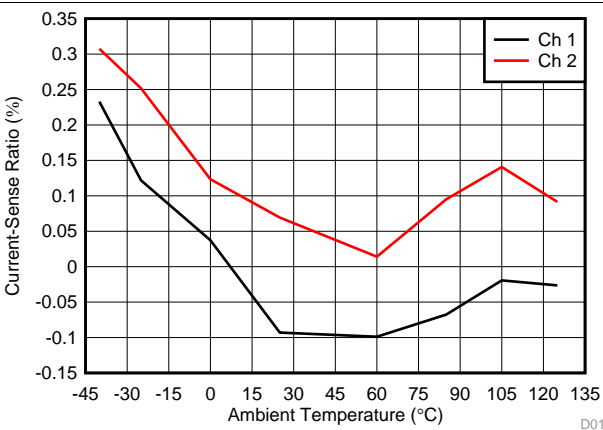
Figure 14. Current-Sense Ratio at 2 mA
