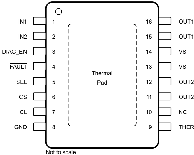
PWP PowerPAD Package 16-Pin HTSSOP With Exposed Thermal Pad TPS2H000-Q1 Version B Top View
