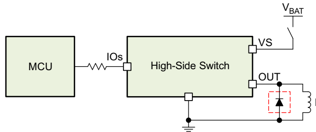
Figure 34. Protection for Loss of Power Supply
