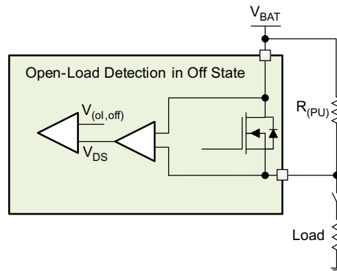
Figure 32. Open-Load Detection in Off-State
