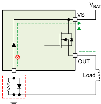
Figure 36. Reverse-Current External Protection, Method 2
