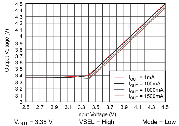
Figure 38. TPS61281A DC Output Voltage vs Input Voltage
