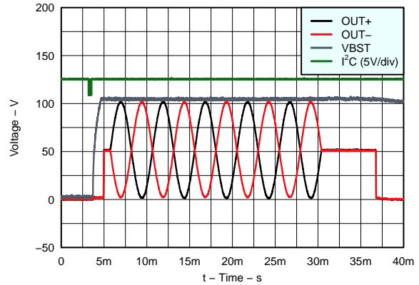
Figure 10. Typical Waveform
