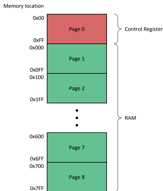
Figure 24. Page Structure
