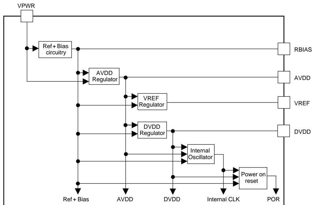
Figure 7. Power-Supply Block
