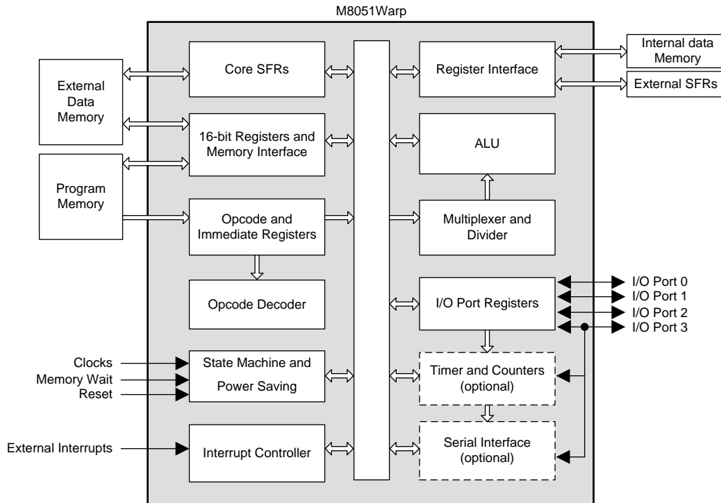
Figure 23. 8051W Core
