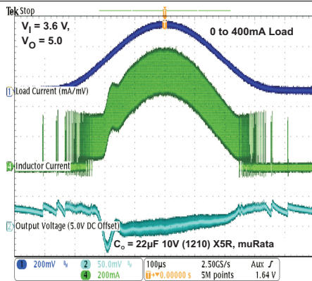
Figure 35. AC Load Transient Response
