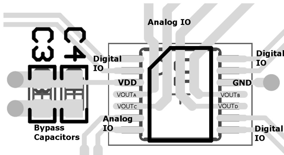
Figure 60. Layout Diagram
