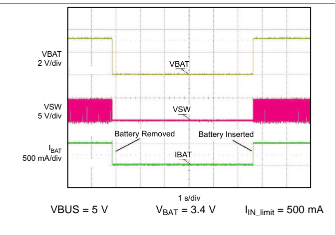
Figure 31. Battery Insertion/Removal (32-s Mode)
