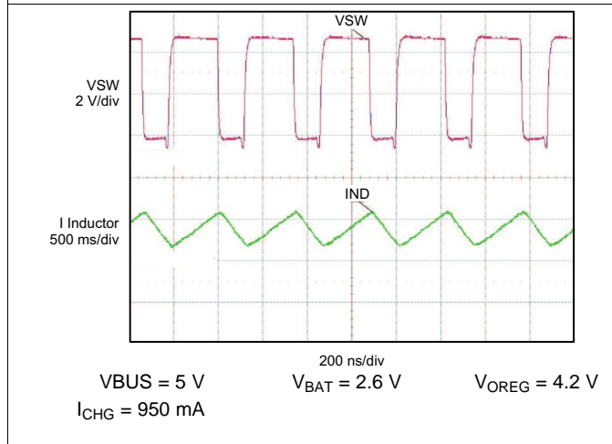
Figure 32. PWM Charging Waveforms
