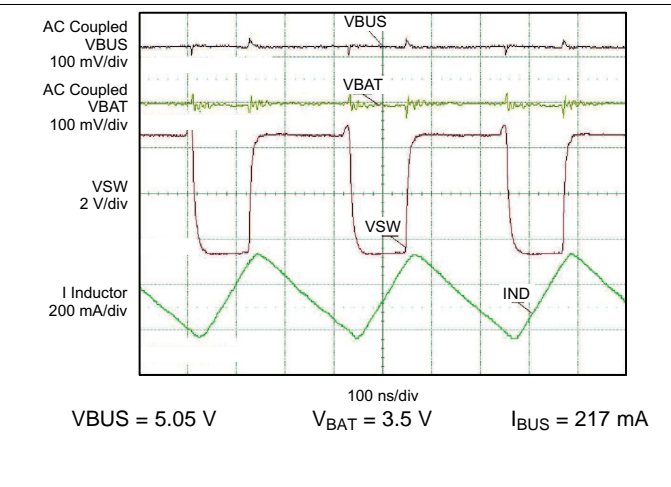
Figure 33. Boost Waveform (PWM Mode)
