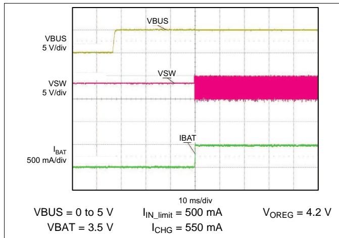
Figure 30. Adapter Insertion (32-s Mode)
