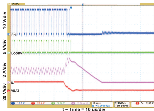
Figure 9. Battery Insertion
