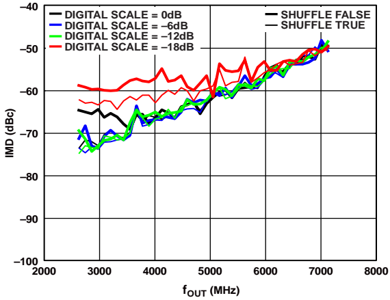
Figure 48. IMD vs. f_{OUT} over Digital Scale
