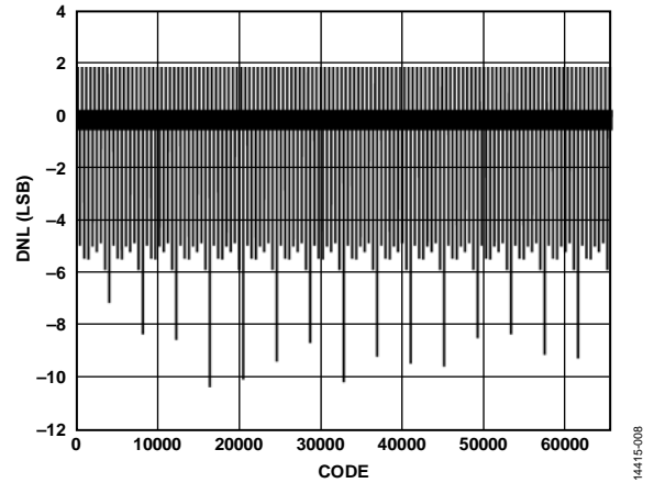
Figure 8. DNL, I_{OUTFS} = 20\text{ mA}
