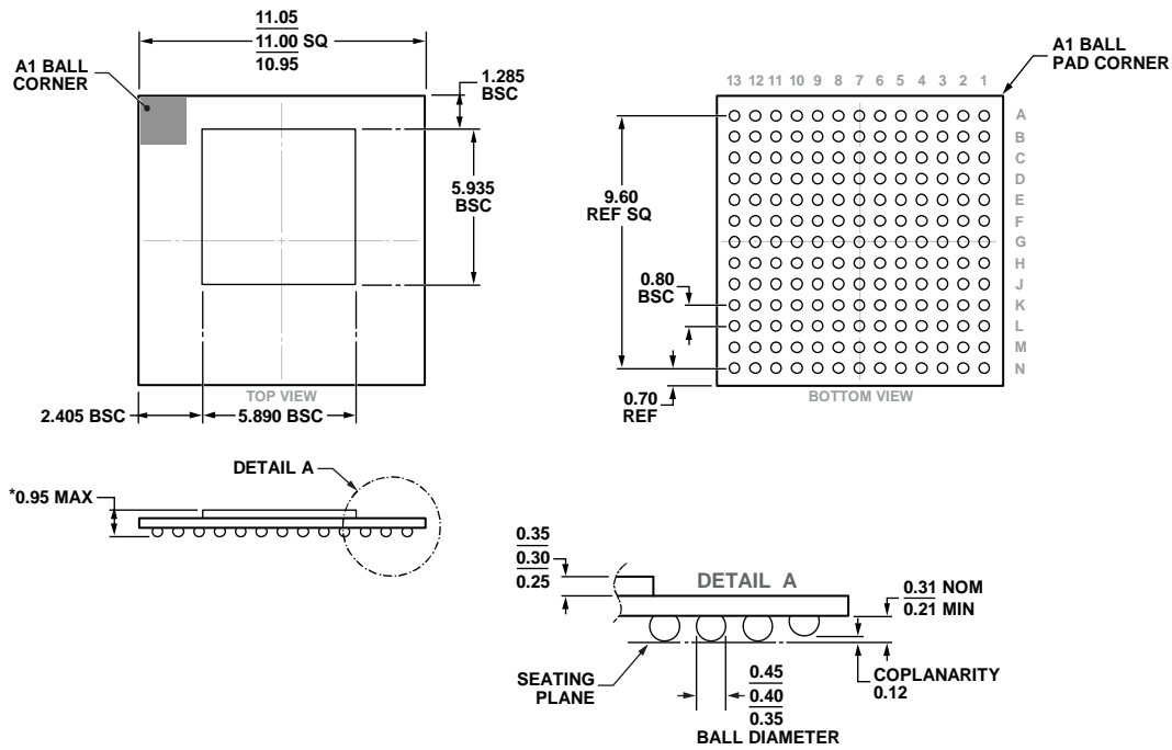
Figure 141. 169-Ball Chip Scale Package Ball Grid Array [CSP_BGA] (BC-169-2) Dimensions shown in millimeters
