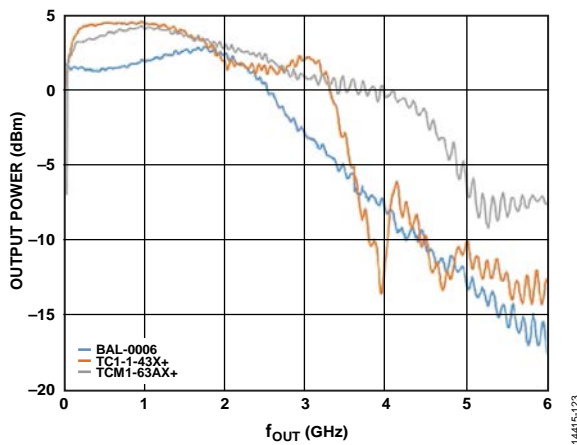
Figure 137. Measured DAC Output Response; f DAC = 6 GSFS
