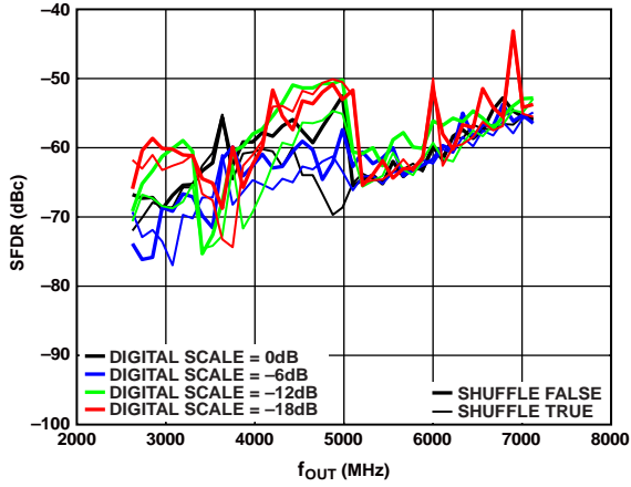
Figure 47. SFDR vs. f_{OUT} over Digital Scale
