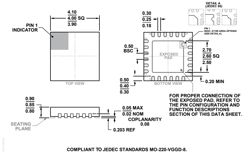
COMPLIANT TO JEDEC STANDARDS MO-220-VGGD-8. Figure 23. 24-Lead Lead Frame Chip Scale Package [LFCSP] 4 mm × 4 mm Body and 0.85 mm Package Height (HCP-24-3) Dimensions shown in millimeters
