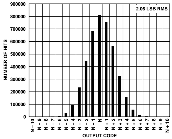
Figure 51. Input-Referred Noise Histogram
