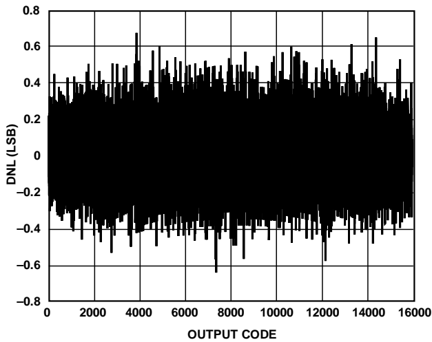
Figure 50. DNL, f_{IN} = 15 MHz
