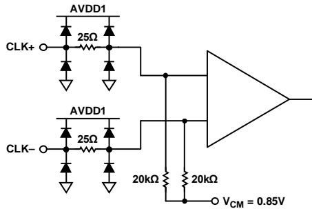
Figure 53. Analog Inputs
