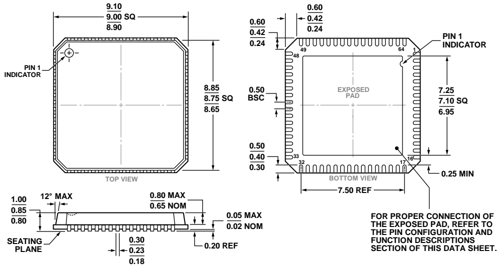
COMPLIANT TO JEDEC STANDARDS MO-220-VMM4 Figure 91. 64-Lead Lead Frame Chip Scale Package [LFCSP_VQ] 9 mm × 9 mm Body, Very Thin Quad (CP-64-3) Dimensions shown in millimeters
