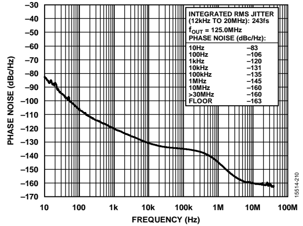
Figure 12. Absolute Phase Noise (PLL1, Configuration 4, HCSSL Mode, f_r = 125\text{ MHz} , f_{OUT} = 125\text{ MHz} , f_{COMP} = 19.2\text{ MHz} TCXO, f_{SYS} = 52\text{ MHz} Crystal, 0.1 Hz DPLL BW, Phase Buildout Mode)
