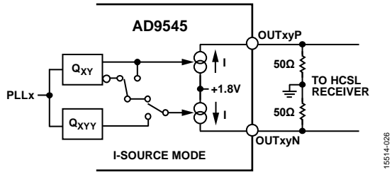
Figure 32. HCSSL Output, V_{p-p} \approx 750 mV per Leg ( I = 15 mA)
