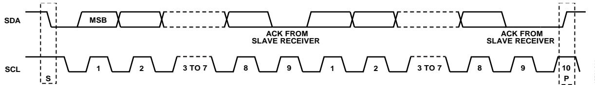
Figure 62. Acknowledge Bit
