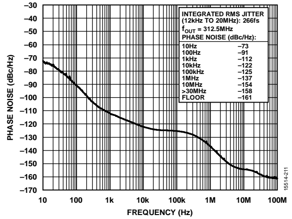
Figure 13. Absolute Phase Noise (PLL1, Configuration 5, HCSSL Mode, f_r = 25\text{ MHz} , f_{OUT} = 312.5\text{ MHz} , f_{SYS} = 52\text{ MHz} Crystal, 50 Hz DPLL BW, Phase Buildout Mode)
