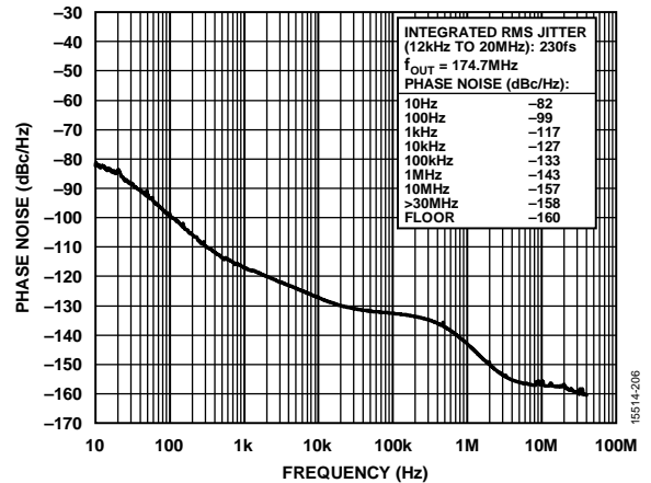
Figure 8. Absolute Phase Noise (PLL0, Configuration 6, HCSSL Mode, f_r = 155.52\text{MHz} , f_{OUT} = 174.7\text{MHz} , f_{SYS} = 52\text{MHz} Crystal, 50 Hz DPLL BW, Phase Buildout Mode)
