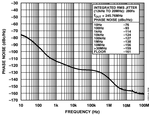
Figure 10. Absolute Phase Noise (PLL1, Configuration 2, HCSSL Mode, f_r = 30.72\text{ MHz} , f_{OUT} = 245.76\text{ MHz} , f_{SYS} = 52\text{ MHz} Crystal, 50 Hz DPLL BW)
