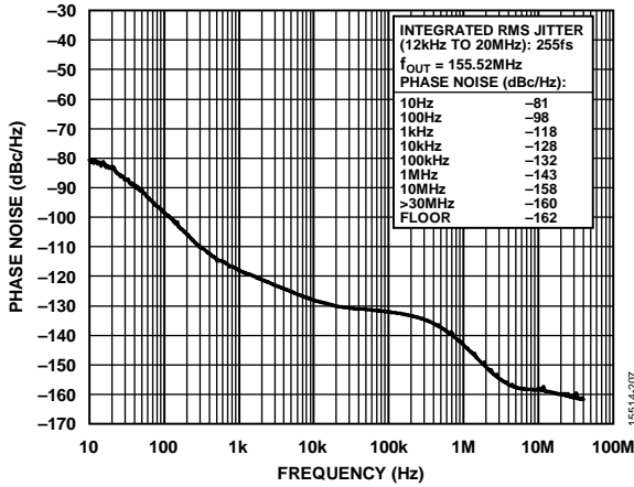
Figure 9. Absolute Phase Noise (PLL1, Configuration 1, HCSSL Mode, f_r = 38.88\text{ MHz} , f_{OUT} = 155.52\text{ MHz} , f_{SYS} = 52\text{ MHz} Crystal, 50 Hz DPLL BW)
