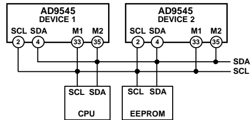
Figure 53. Level 2 Multidevice Configuration
