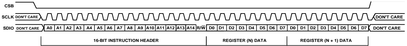
Figure 58. Serial Control Port Write—LSB First, Address Increment, Two Bytes of Data
