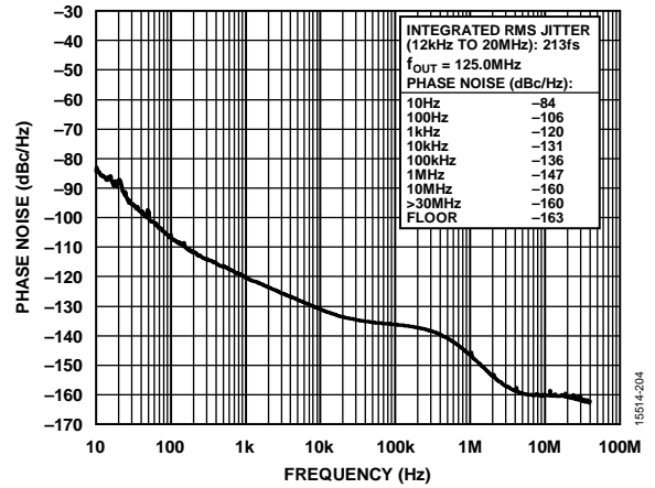
Figure 6. Absolute Phase Noise (PLL0, Configuration 4, HCSSL Mode, f_r = 125\text{MHz} , f_{OUT} = 125.0\text{MHz} , f_{COMP} = 19.2\text{MHz} TCXO, f_{SYS} = 52\text{MHz} Crystal, 0.1 Hz DPLL BW, Phase Buildout Mode)
