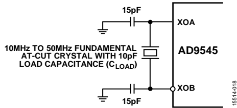
Figure 23. System Clock Input (XOA/XOB) in Crystal Mode (the 15 pF Shunt Capacitors Shown Here Each Must Equal 2 \times (C_{LOAD} - C_{STRAY}) , Where Typical C_{STRAY} = 2 \text{ pF to } 5 \text{ pF} )
