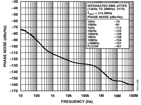
Figure 7. Absolute Phase Noise (PLL0, Configuration 5, HCSSL Mode, f_r = 25\text{MHz} , f_{OUT} = 312.5\text{MHz} , f_{SYS} = 52\text{MHz} Crystal, 50 Hz DPLL BW, Phase Buildout Mode)
