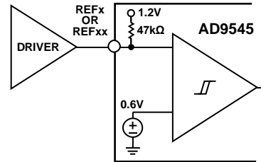
Figure 27. Single-Ended Internal Pull-Up Mode
