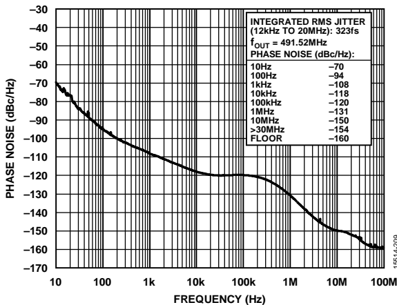
Figure 11. Absolute Phase Noise (PLL1, Configuration 3, HCSSL Mode, f_r = 1\text{ Hz} , f_{OUT} = 491.52\text{ MHz} , f_{COMP} = 19.2\text{ MHz} TCXO, f_{SYS} = 52\text{ MHz} Crystal, 50 MHz DPLL BW)
