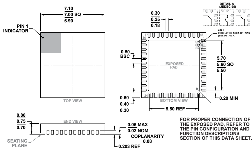
COMPLIANT TO JEDEC STANDARDS MO-220-WKKD-4. Figure 66. 48-Lead Lead Frame Chip Scale Package [LFCSP] 7 mm x 7 mm Body and 0.75 mm Package Height (CP-48-13) Dimensions shown in millimeters
