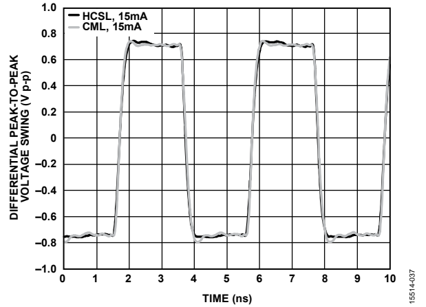
Figure 18. 245.76 MHz Output Waveform for 15 mA Driver Settings; HCSL Drivers Terminated 50 Ω to GND per Figure 32; CML Drivers Terminated 50 Ω to 1.8 V per Figure 33
