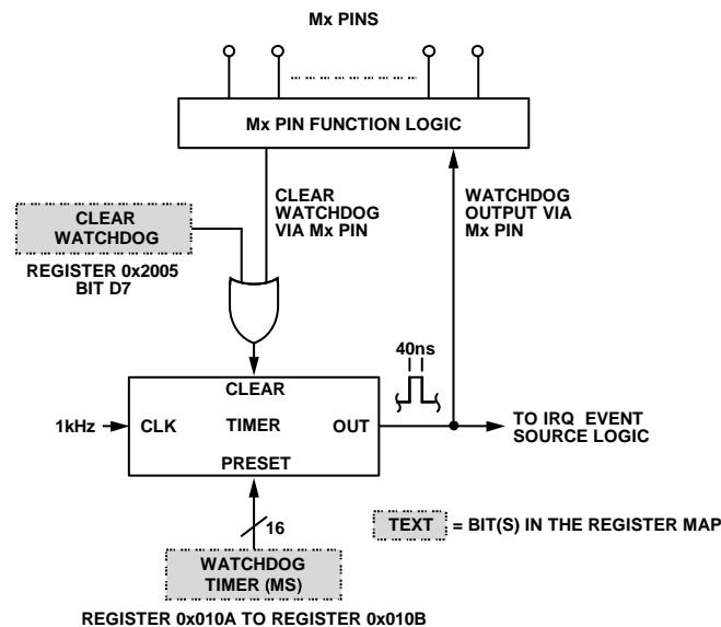
Figure 49. Watchdog Timer
