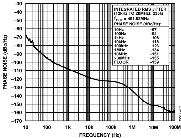
Figure 5. Absolute Phase Noise (PLL0, Configuration 3, HCSSL Mode, f_r = 1\text{Hz} , f_{OUT} = 491.52\text{MHz} , f_{COMP} = 19.2\text{MHz} TCXO, f_{SYS} = 52\text{MHz} Crystal, 50 MHz DPLL BW)
