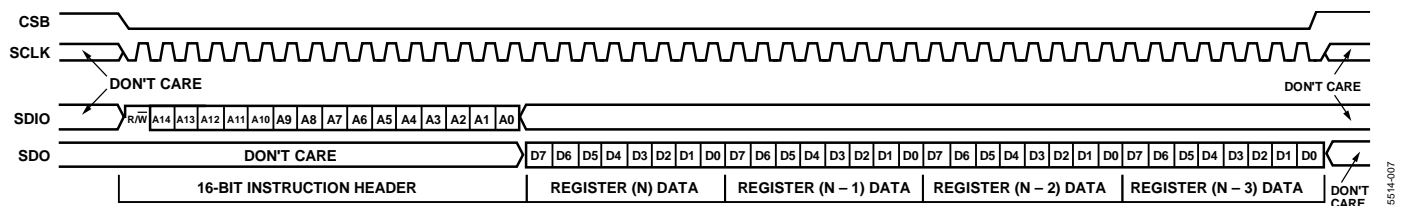
Figure 55. Serial Control Port Read—MSB First, Address Decrement, Four Bytes of Data
