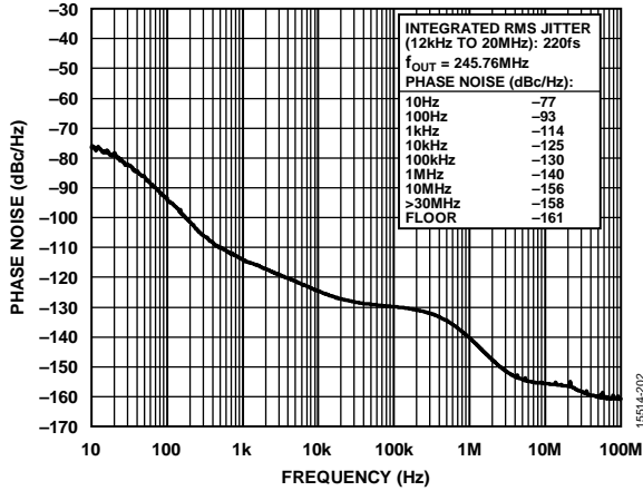
Figure 4. Absolute Phase Noise (PLL0, Configuration 2, HCSSL Mode, f_r = 30.72\text{MHz} , f_{OUT} = 245.76\text{MHz} , f_{SYS} = 52\text{MHz} Crystal, 50 Hz DPLL BW)
