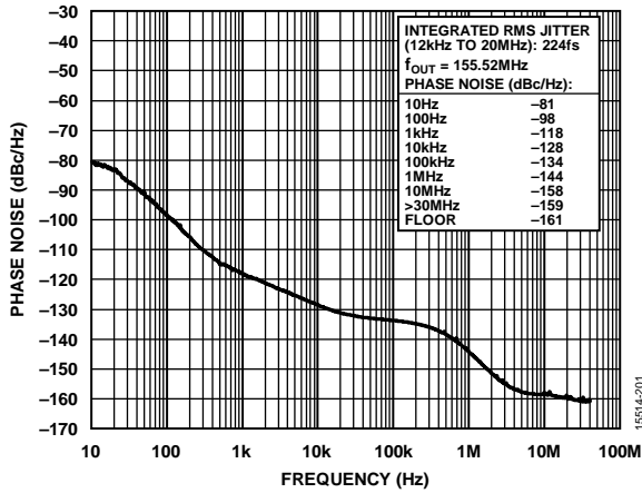
Figure 3. Absolute Phase Noise (PLL0, Configuration 1, HCSSL Mode, f_r = 38.88\text{MHz} , f_{OUT} = 155.52\text{MHz} , f_{SYS} = 52\text{MHz} Crystal, 50 Hz DPLL BW)
