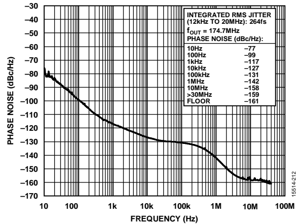
Figure 14. Absolute Phase Noise (PLL1, Configuration 6, HCSSL Mode, f_r = 155.52\text{ MHz} , f_{OUT} = 174.7\text{ MHz} , f_{SYS} = 52\text{ MHz} Crystal, 50 Hz DPLL BW, Phase Buildout Mode)
