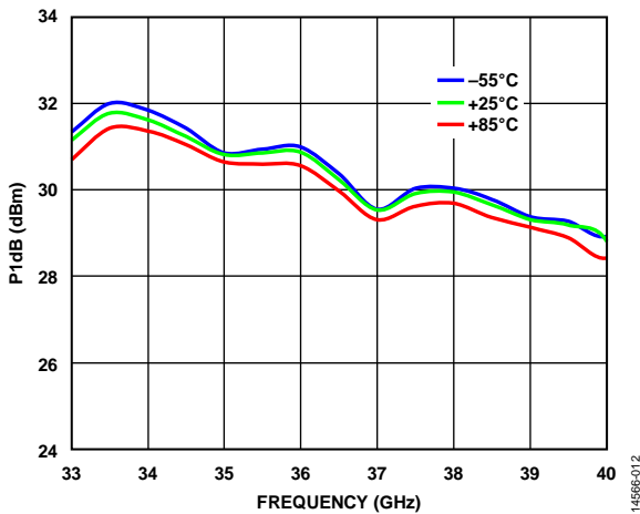
Figure 12. P1dB vs. Frequency at Various Temperatures
