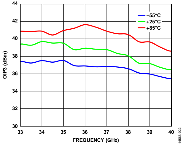
Figure 22. Output IP3 vs. Frequency at Various Temperatures
