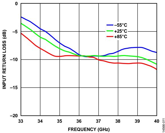
Figure 11. Input Return Loss vs. Frequency at Various Temperatures
