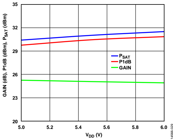
Figure 29. Gain, P1dB, and P_{SAT} vs Supply Voltage ( V_{DD} ) at 36 GHz
