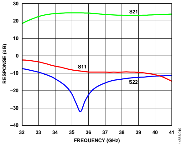
Figure 10. Response Gain and Return Loss vs. Frequency
