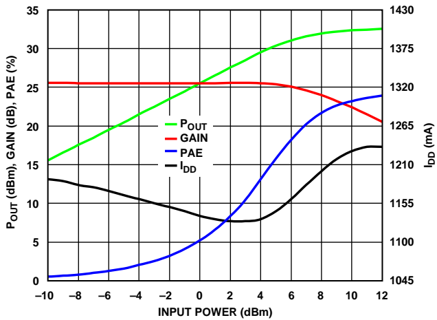
Figure 18. Power Compression at 34 GHz ( I_{DD} is Drain Current With RF Power Applied)
