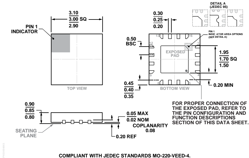
Figure 25. 16-Lead Lead Frame Chip Scale Package [LFCS] 3 mm x 3 mm Body and 0.85 mm Package Height (HCP-16-1) Dimensions shown in millimeters
