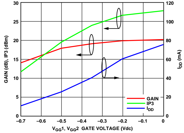
Figure 20. Gain, IP3, and I_{DD} vs. V_{GG1} , V_{GG2} Gate Voltage at 7 GHz (Board Loss Removed from Gain Measurement, Data Taken at V_{DD1} = V_{DD2} = 3 V)
