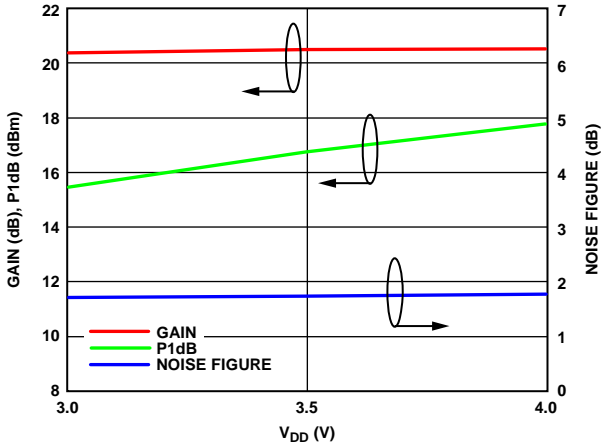
Figure 18. Gain, P1dB, and Noise Figure vs. Supply Voltage ( V_{DD} ) at 7 GHz (Board Loss Removed from Gain, Power and Noise Figure Measurement)
