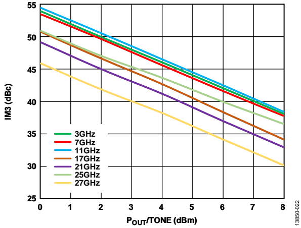
Figure 22. Output IM3 vs. P_{out}/Tone for Various Frequencies at V_{DD} = 7.5 V
