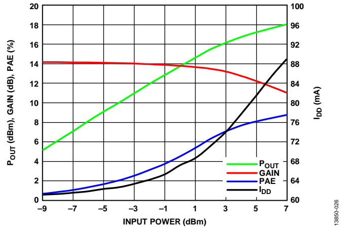
Figure 26. Power Compression at 15 GHz
