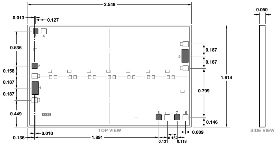
Figure 46. 8-Pad Bare Die [CHIP] (C-8-8) Dimensions shown in millimeters
