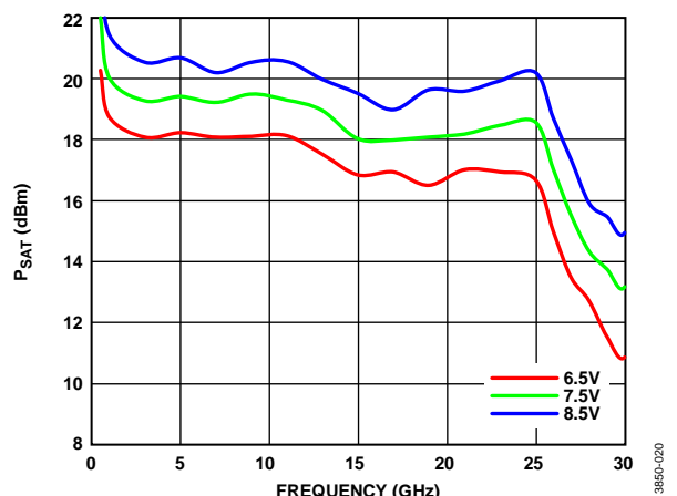
Figure 20. P_{SAT} vs. Frequency at Various Supply Voltages
