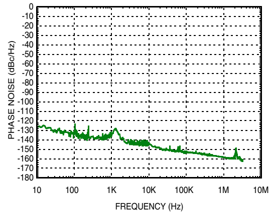
Phase Noise at P1dB at 8 GHz vs. Frequency
