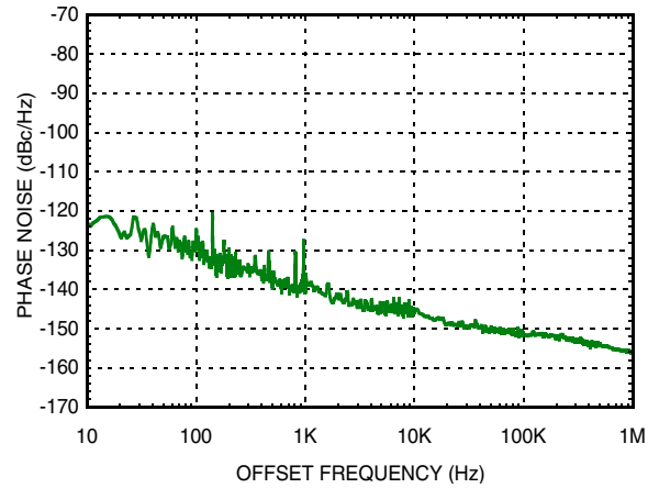
Phase Noise @ P1dB at , 8GHz vs. Frequency
