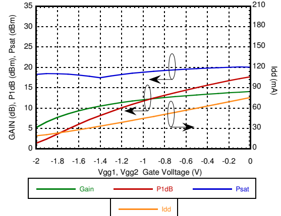
Gain, Power & Idd vs. Gate Voltage @ 10 GHz
