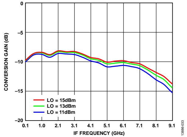
Figure 33. Conversion Gain vs. IF Frequency at Various LO Power Levels, TA = 25°C
