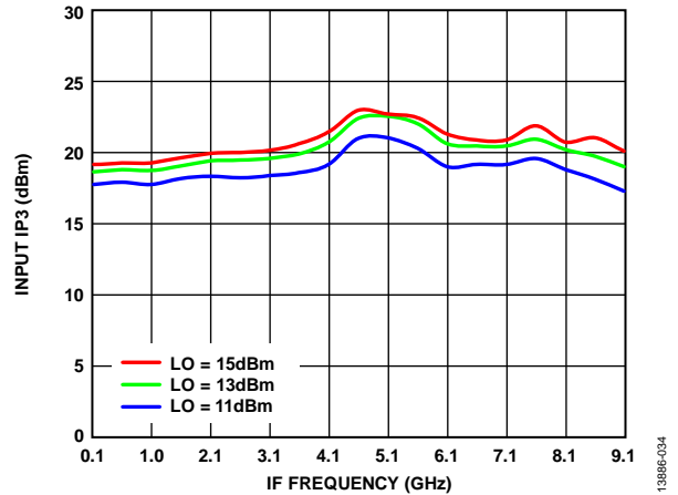
Figure 34. Input IP3 vs. IF Frequency at Various LO Power Levels, TA = 25°C
