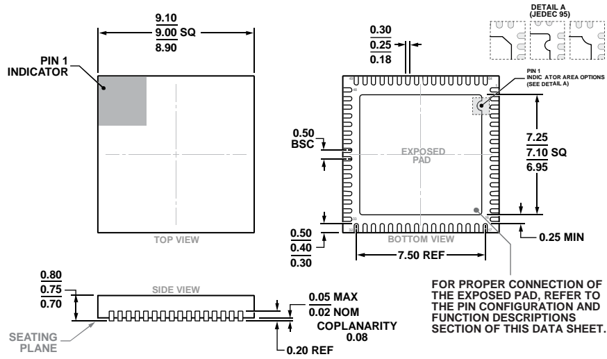
Figure 61. 64-Lead Lead Frame Chip Scale Package [LFCSP] 9 mm × 9 mm Body and 0.75 mm Package Height (CP-64-12)
