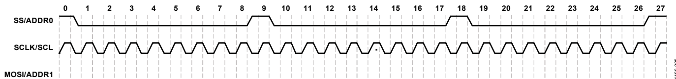
Figure 33. Example of SPI Slave Mode Initialization Sequence Using Dummy Writes
