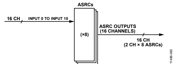
Figure 56. Example ASRC Routing, Bypassing DSP Core
