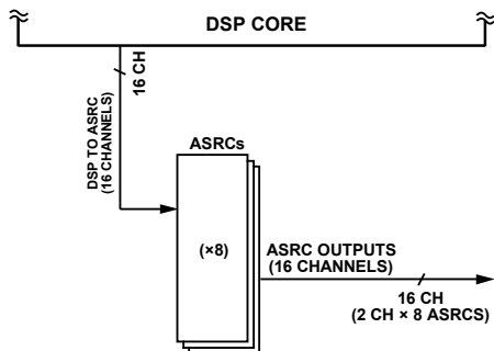
Figure 53. Example ASRC Routing for Asynchronous Serial Output from the DSP Core
