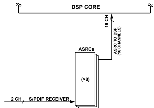
Figure 50. Example ASRC Routing for Asynchronous Input to the DSP Core
