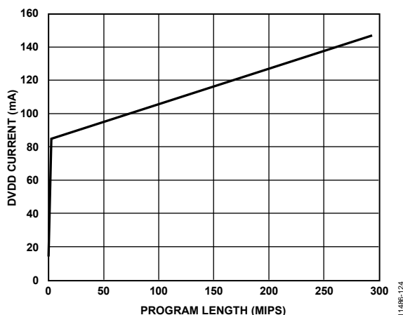
Figure 24. ADAU1467 Typical DVDD Current Draw vs. Program MIPS at an Ambient Temperature of 25°C and a Sample Rate of 48 kHz
