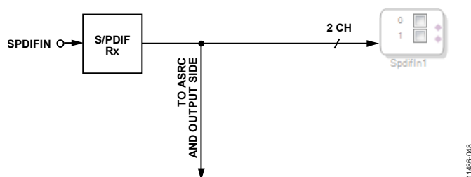
Figure 44. S/PDIF Receiver Direct Input Mapping to DSP in SigmaStudio
