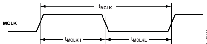
Figure 2. Master Clock Input Timing Specifications
