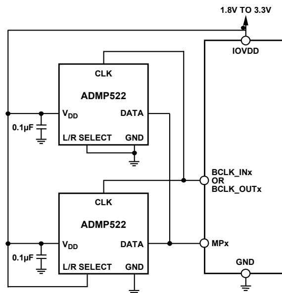
Figure 71. Example Stereo PDM Microphone Input Circuit
