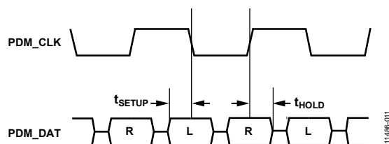
Figure 10. PDM Timing Diagram
