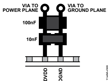
Figure 81. Layout for Multiple Power Supply Bypass Capacitors
