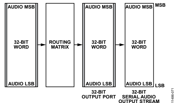
Figure 66. 32-Bit Serial Output Example
