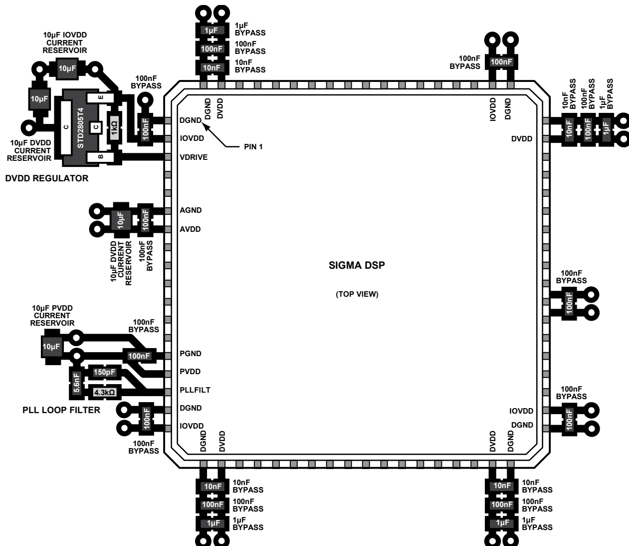
Figure 87. Supporting Component Placement and Layout
