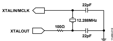
Figure 14. Crystal Resonator Circuit
