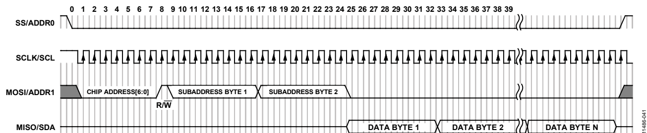
Figure 37. SPI Slave Read Clocking (Burst Read Mode, N Bytes)
