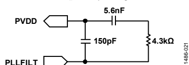
Figure 16. PLL Filter
