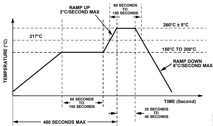
Figure 88. Soldering Profile
