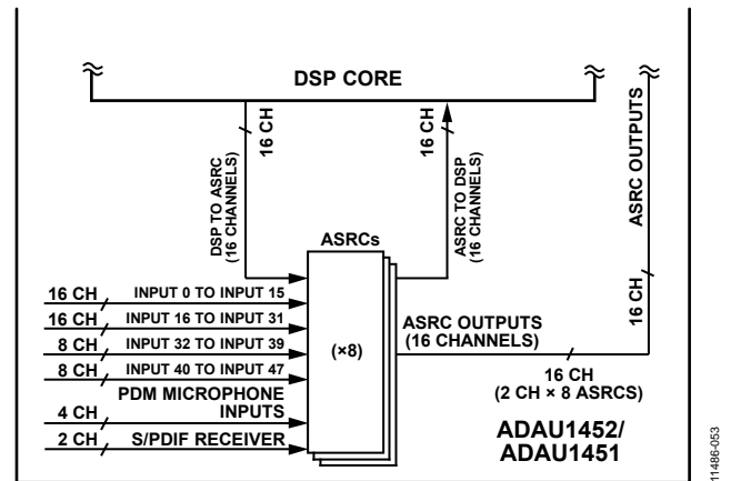
Figure 49. Channel Routing to ASRC Inputs
