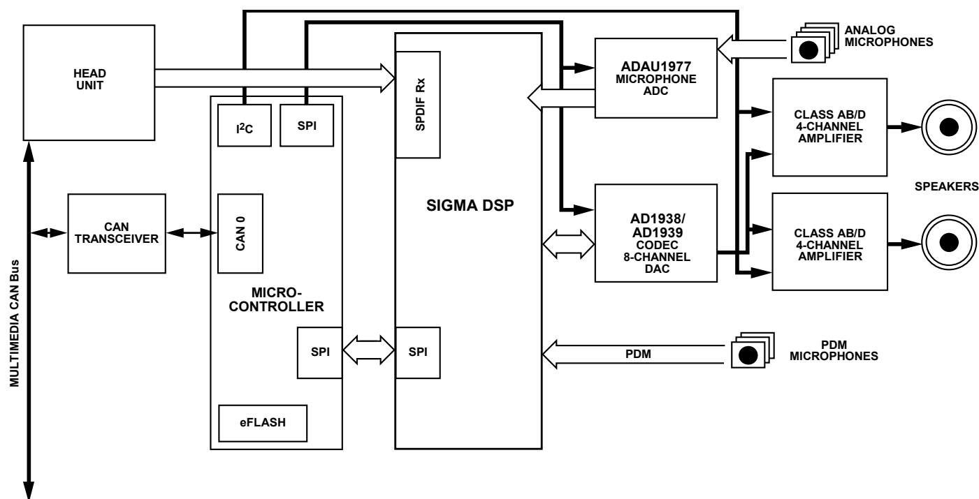
Figure 86. Automotive Infotainment Amplifier Block Diagram
