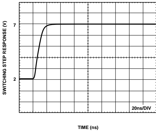
Figure 14. Data Switching Step Response (Rising Edge), 5 V Step, C_L = 200 pF, INV = LOW
