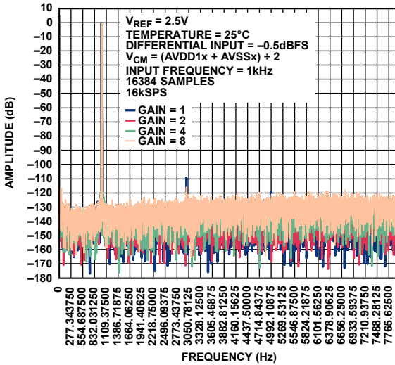
Figure 27. FFT Plot, High Resolution Mode, Input Frequency ( f_{IN} ) = 1 kHz
