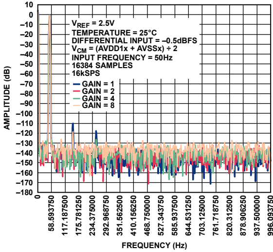
Figure 26. FFT Plot at 16 kSPS, High Resolution Mode, Input Frequency ( f_{IN} ) = 50 Hz (This Plot is a Close Up Perspective of the Original Data)
