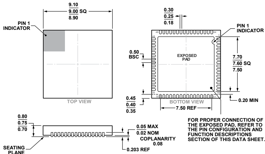
Figure 122. 64-Lead Lead Frame Chip Scale Package [LFCSP] 9 mm × 9 mm Body and 0.75 mm Package Height (CP-64-15)
