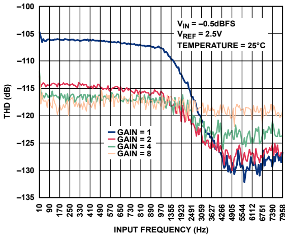
Figure 28. THD vs. Input Frequency at 8 kSPS, High Resolution Mode
