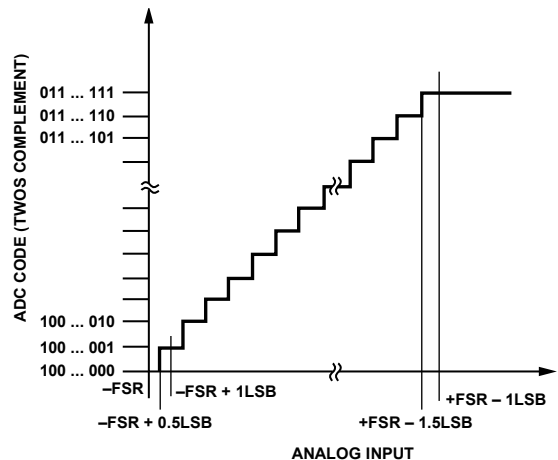
Figure 90. Transfer Function
