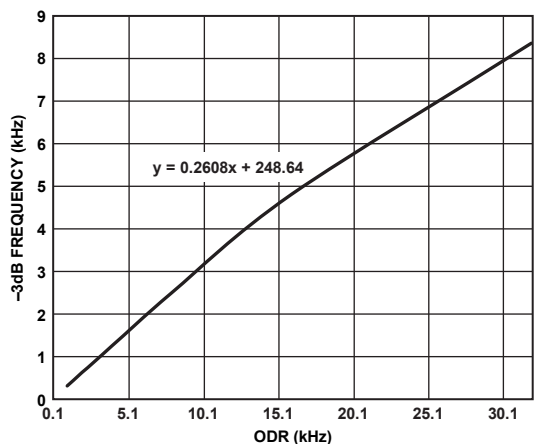
Figure 111. -3 dB Correction Factor
