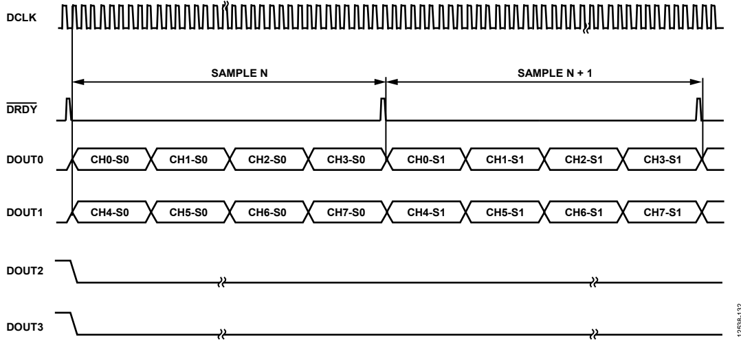
Figure 116. FORMAT0 = 0, FORMAT1 = 1 —Channel 0 to Channel 3 Share DOUT0 , and Channel 4 to Channel 7 Share DOUT1 (S0 Means Sample 0 and S1 Means Sample 1)
