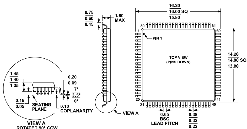
图69. 80引脚薄型四方扁平封装 [LQFP] (ST-80-2)
