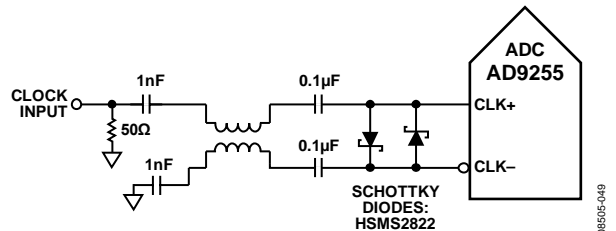
Figure 76. Balun-Coupled Differential Clock (625 MHz)
