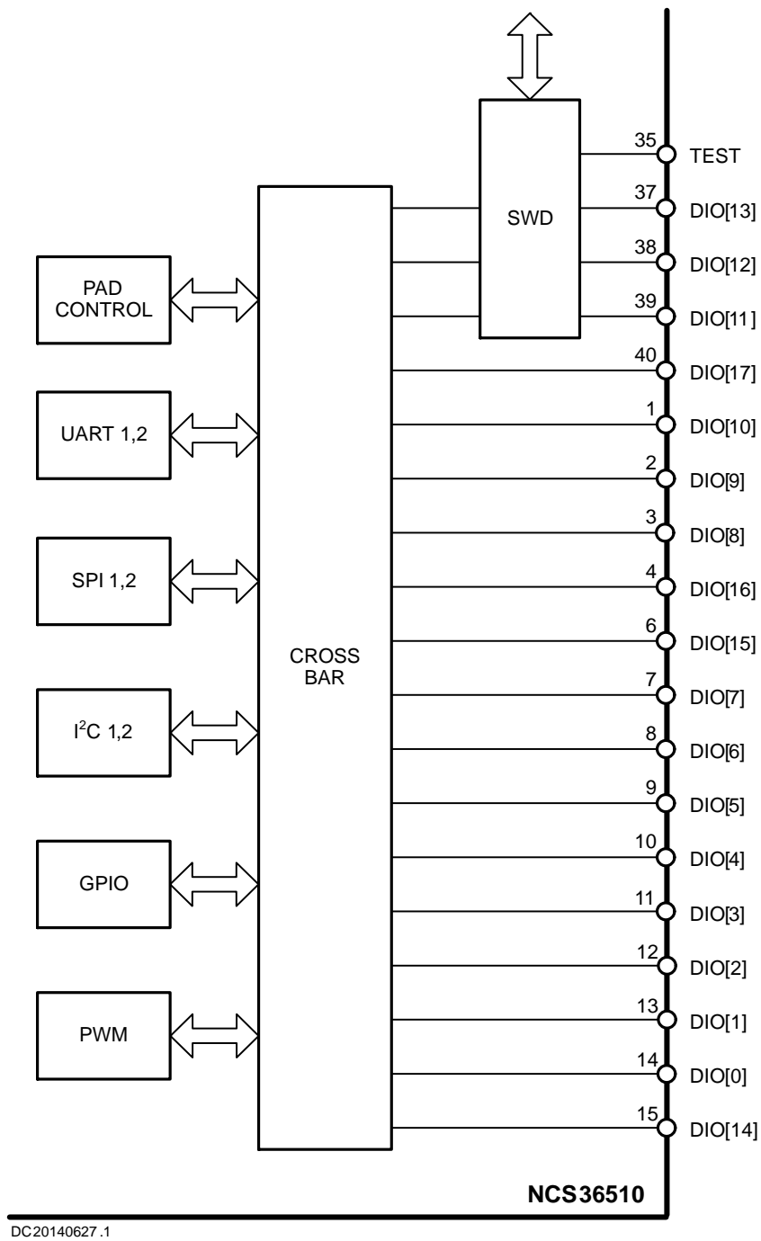
Figure 7. Cross Bar
