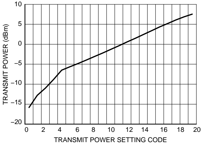
Figure 16. 3 V Mode with Switching Regulator Transmitter Power in CW Mode, 2.4425 GHz
