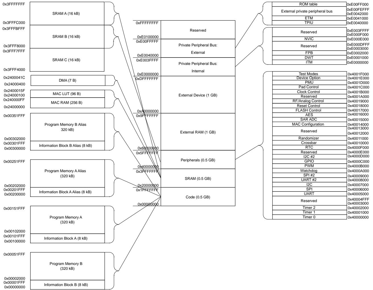
Figure 3. Memory Map
