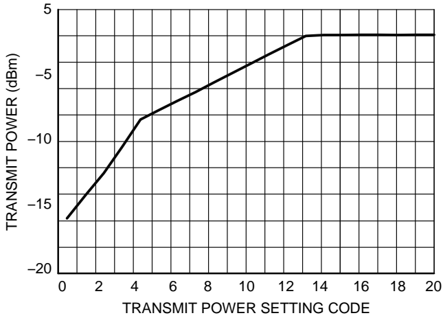
Figure 21. 1 V Mode Transmitter Power in CW Mode, 2.4425 GHz
