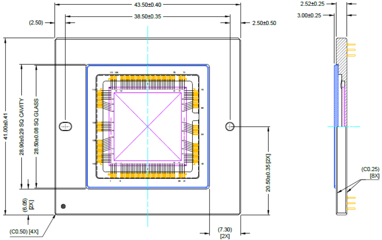
Figure 43. Completed Assembly 1
