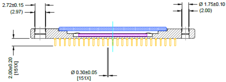
Figure 44. Completed Assembly 2
