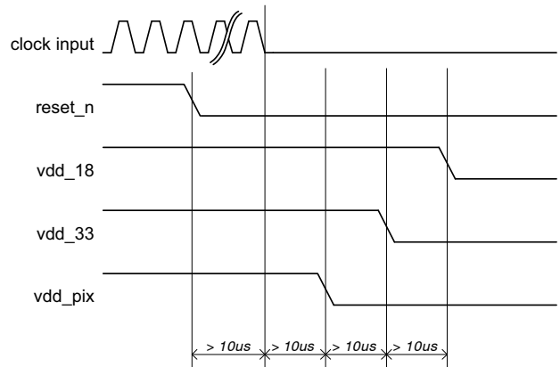
Figure 18. Power Down Sequence
