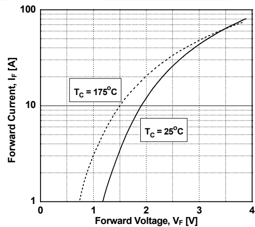
Figure 22. Forward Characteristics
