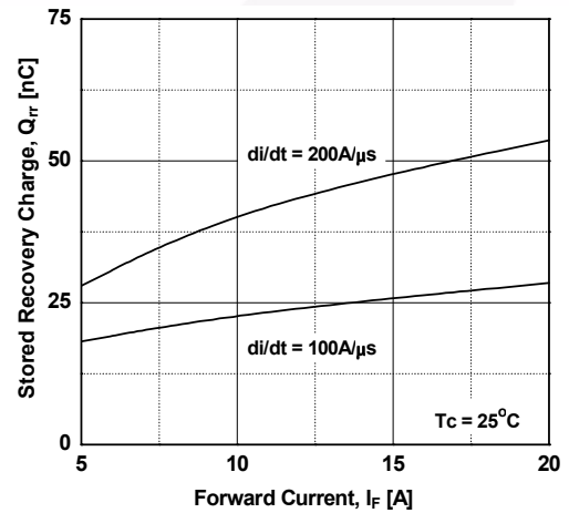
Figure 24. Stored Charge
