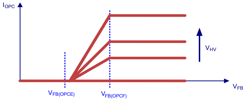
Figure 66. Overpower Protection Current Relation to Feedback Voltage
