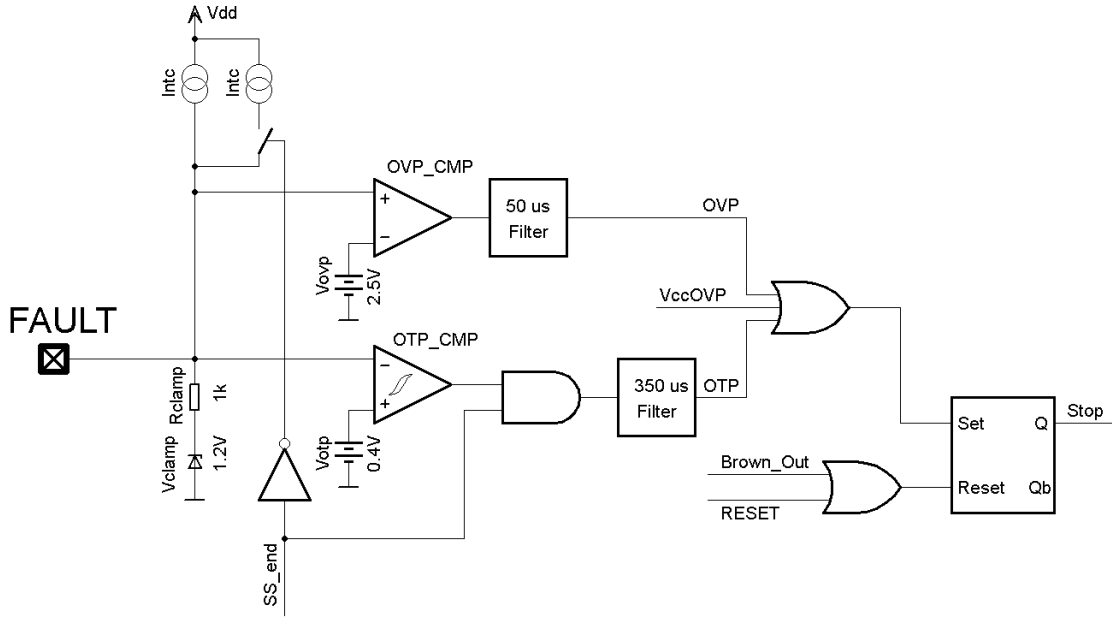
Figure 71. OVP/OTP Detection Schematic
