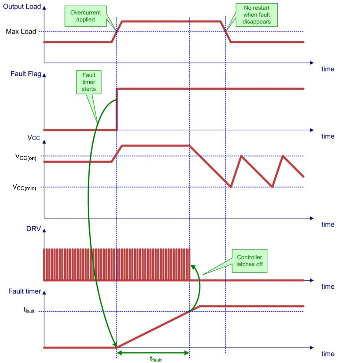
Figure 70. Latched Timer-Based Overcurrent Protection
