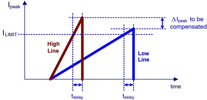
Figure 65. Needs for Line Compensation For True Overpower Protection
