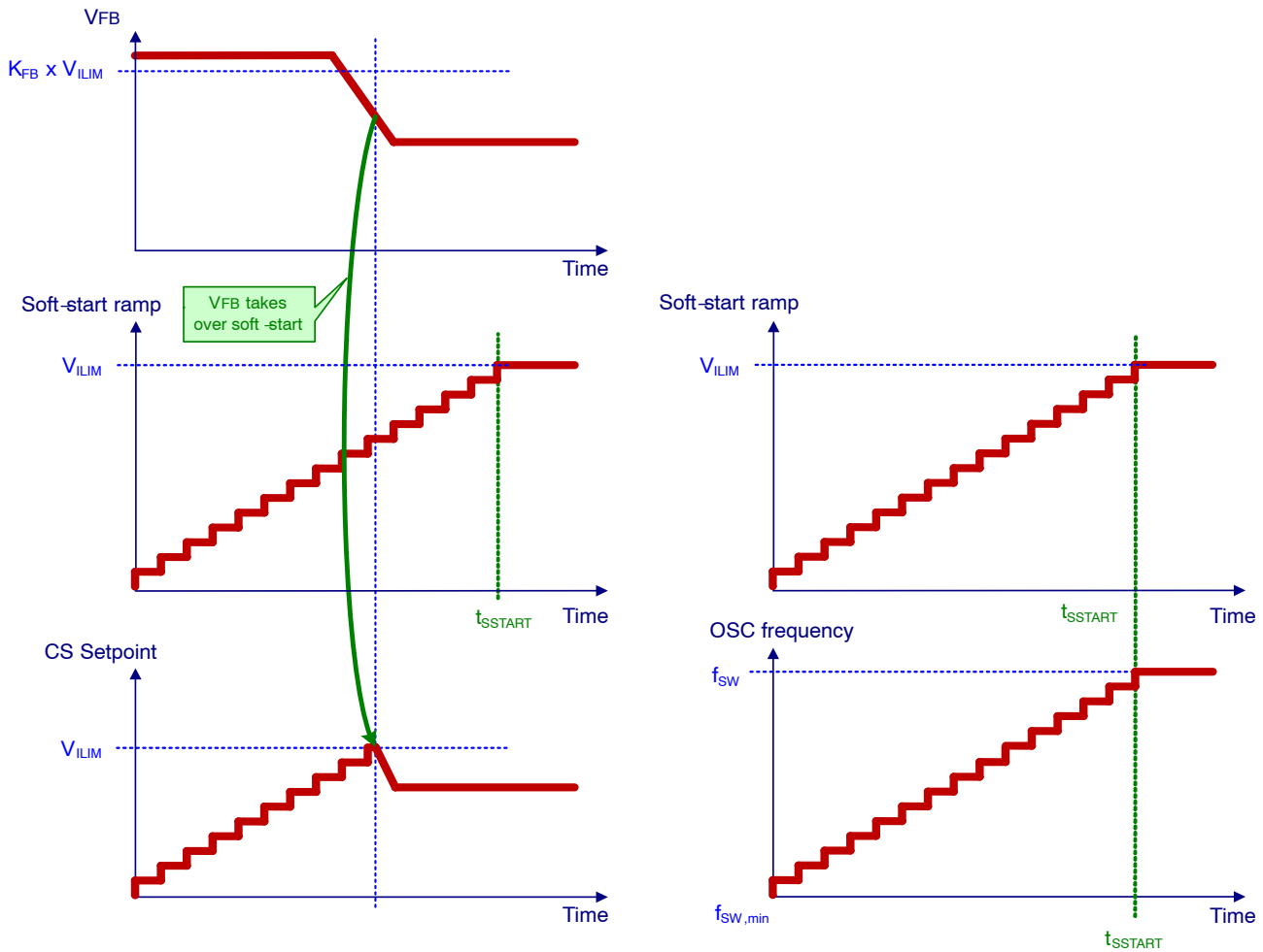
Figure 62. Soft-Start Feature
