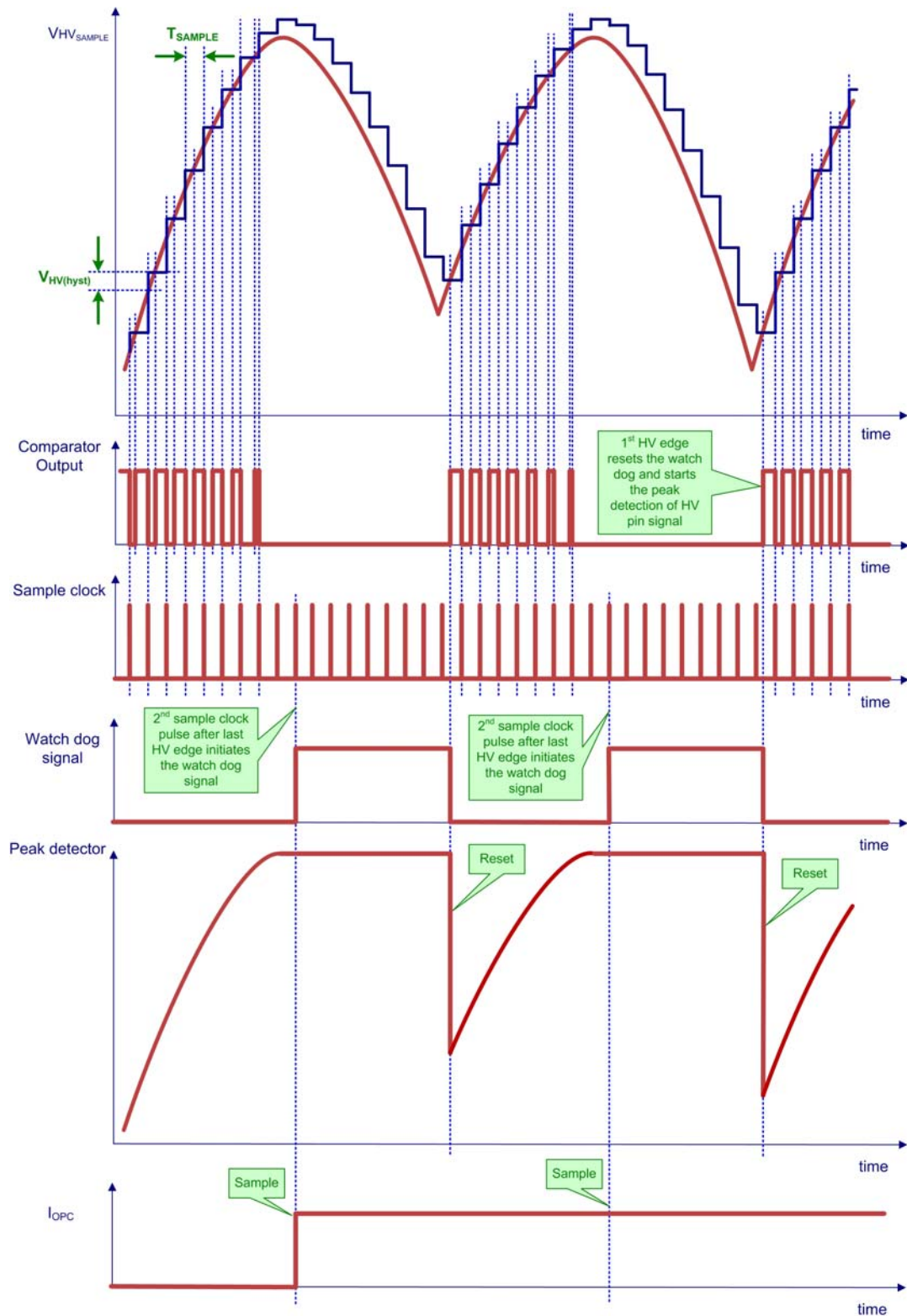
Figure 69. Overpower Compensation Timing Diagram
