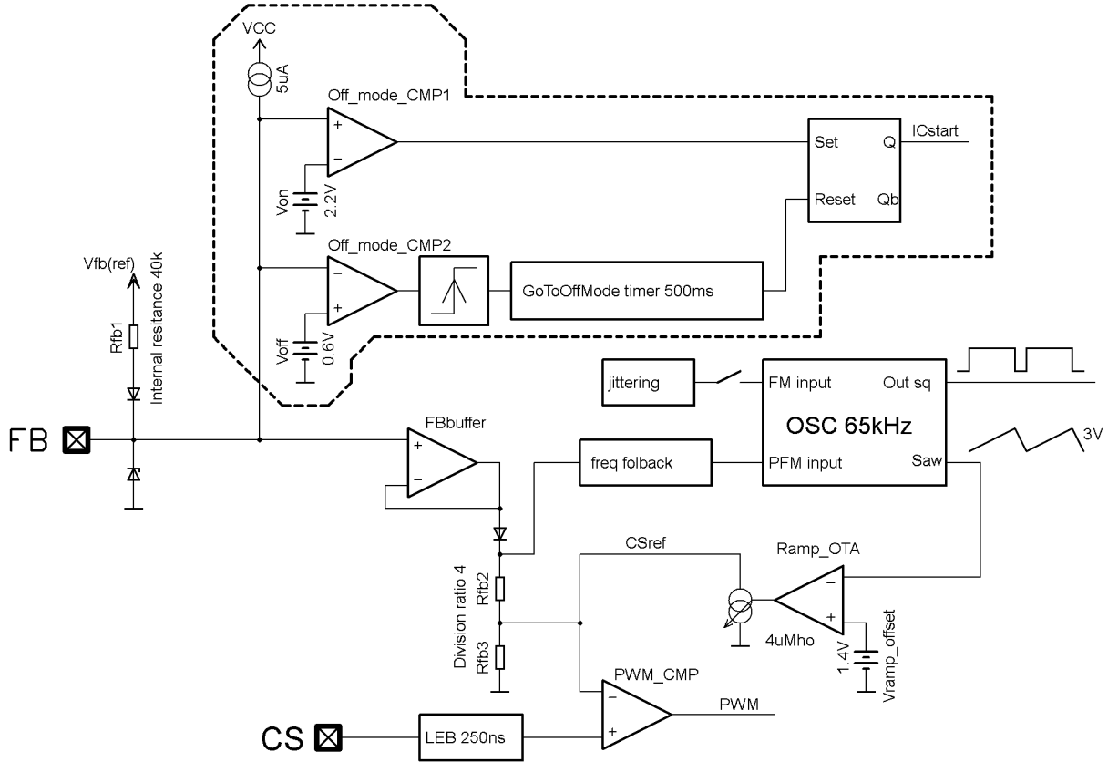
Figure 63. Slope Compensation Block Diagram
