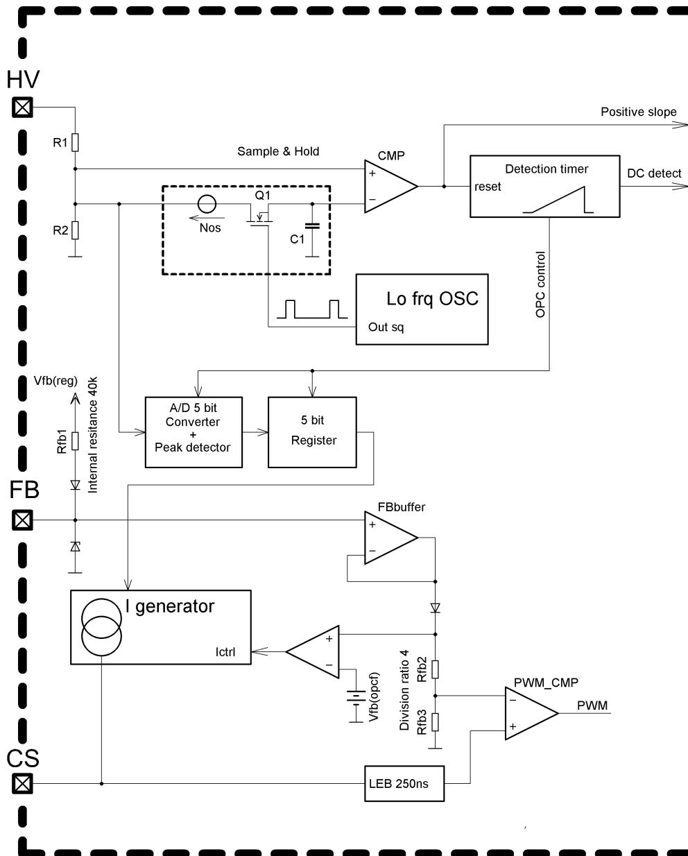
Figure 68. Block Schematic of Overpower Protection Circuit
