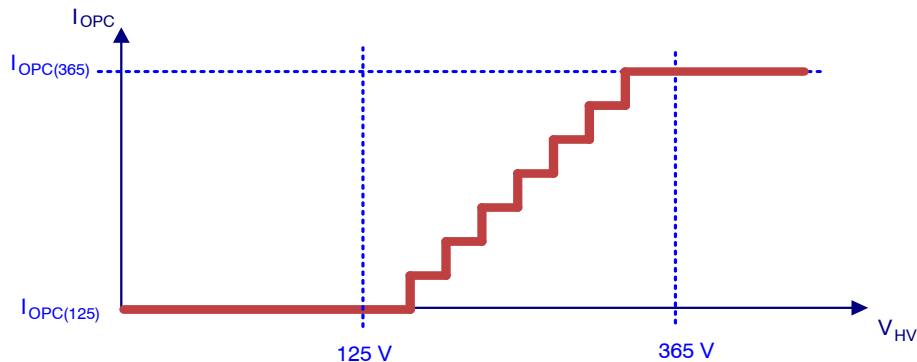
Figure 67. Overpower Protection Current Relation to Peak of Rectified Input Line AC voltage
