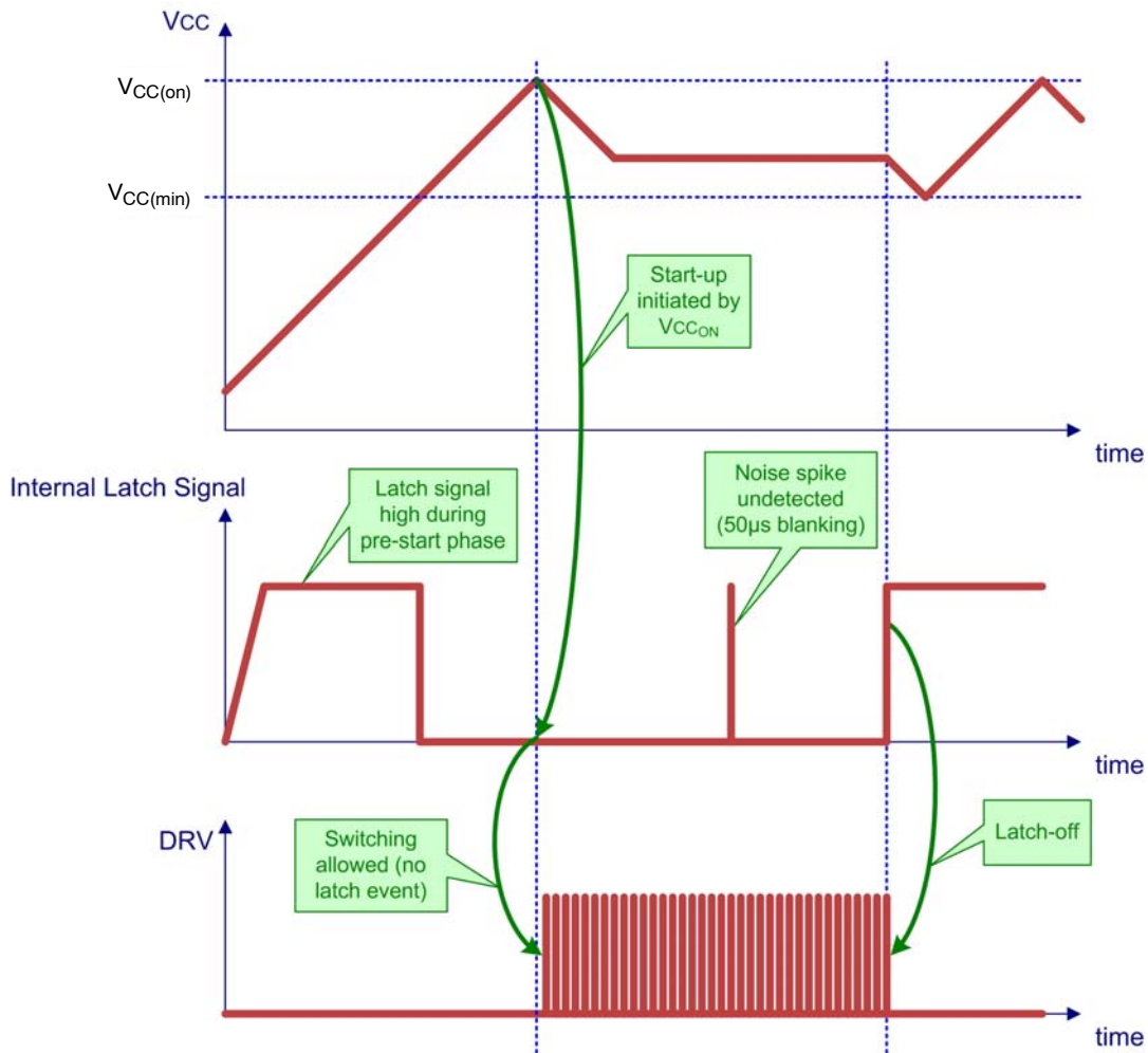
Figure 72. Latch Timing Diagram
