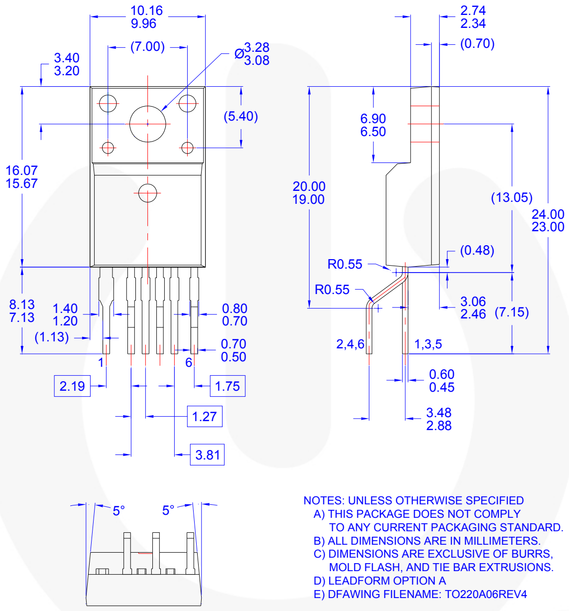
Figure 24. TO-220F-6L (W-Forming)
