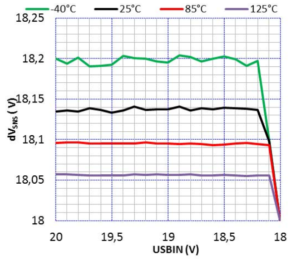
Figure 23. USBSNS Regulation Versus Temperature, VP Low
