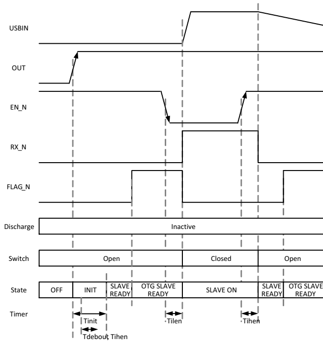
Figure 10. Slave Configuration. Application Of VOUT, Enabling (OTG), Disabling
