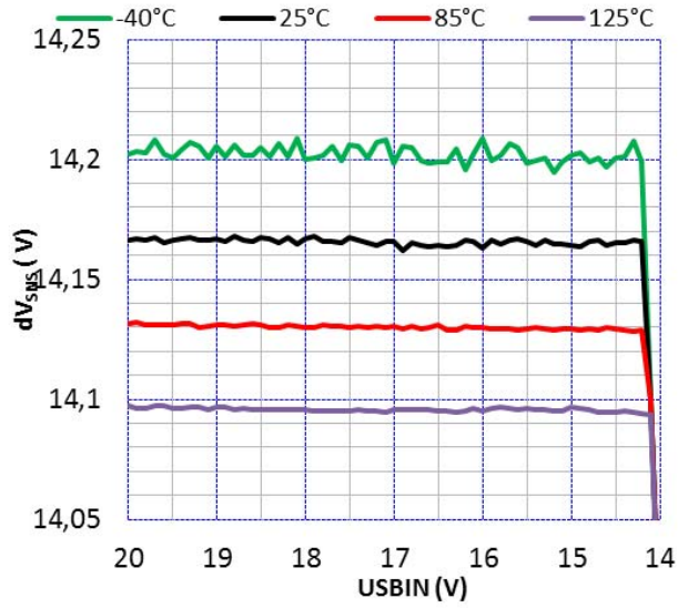
Figure 22. USBSNS Regulation Versus Temperature, VP High
