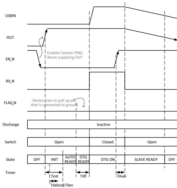
Figure 11. Slave Configuration With FLAG_N To Ground. Simultaneous Enabling Of VOUT And OTG, Simultaneous Disabling
