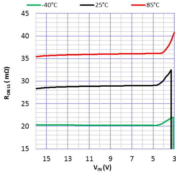
Figure 14. USBIN To Out Mosfet Resistance Versus VIN And Temperature 5A Load
