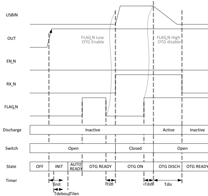
Figure 6. Autonomous Configuration. Application Of VOUT, Enabling (OTG), Disabling
