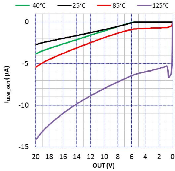
Figure 17. OUT To USBIN Mosfet Leakages, Versus OUT And Temperature
