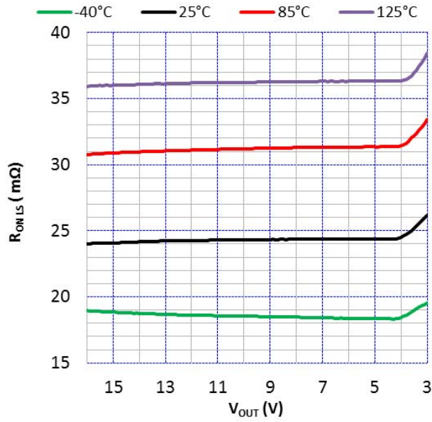
Figure 13. OUT To USBIN Mosfet Resistance Versus VOUT And Temperature No Load
