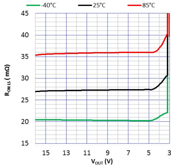
Figure 15. OUT To USBIN Mosfet Resistance Versus Vout And Temperature No Load
