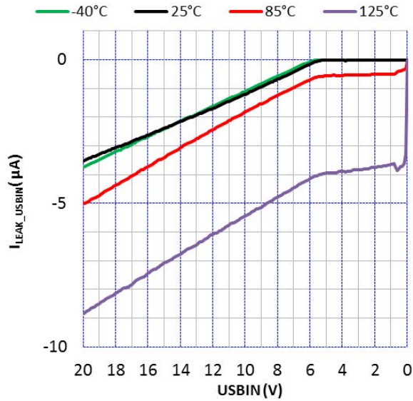
Figure 16. USBIN To Out Mosfet Leakages, Versus USBIN And Temperature
