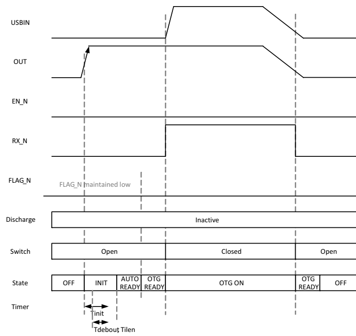
Figure 7. Autonomous Configuration. Application Of VOUT
