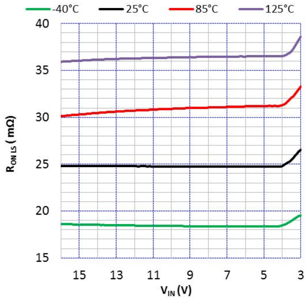
Figure 12. USBIN To OUT MOSFET RESISTANCE Versus VIN And Temperature, No Load
