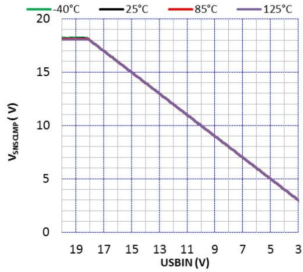
Figure 21. USBSNS Voltage Versus USBIN And Temperature, VP Low
