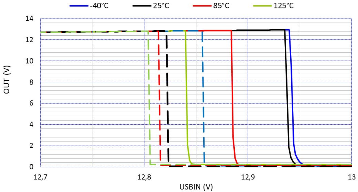
Figure 18. OVLO Threshold And Hysteresis Versus Temperature, VP High
