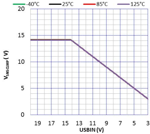
Figure 20. USBSNS Voltage Versus USBIN And Temperature, VP High
