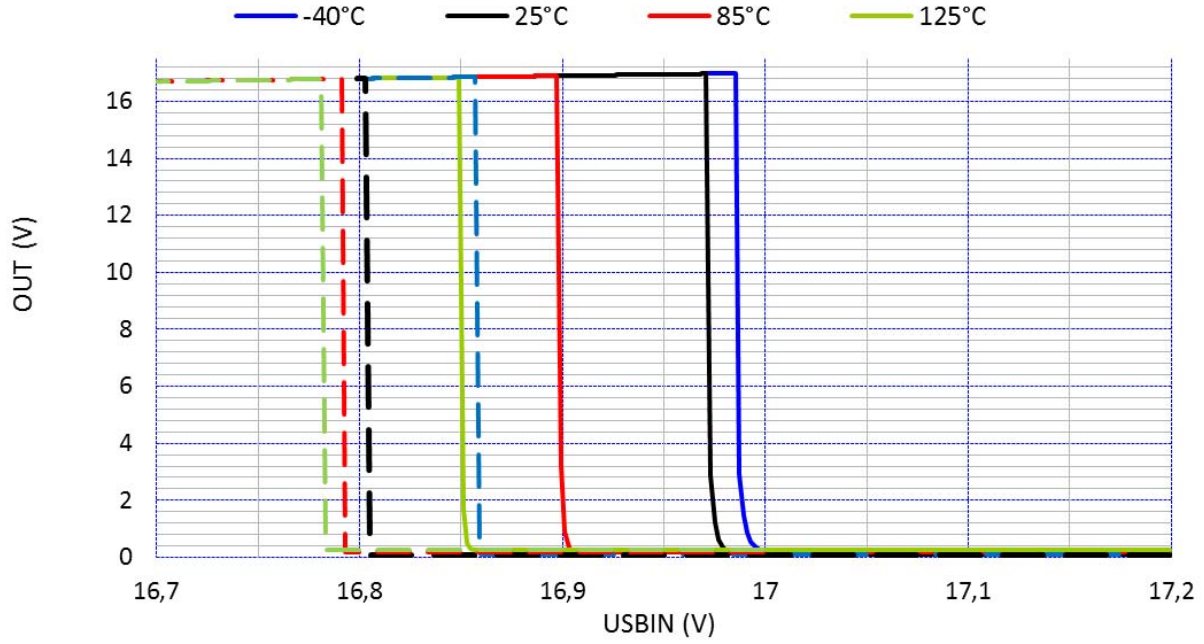
Figure 19. OVLO Threshold And Hysteresis Versus Temperature, VP Low
