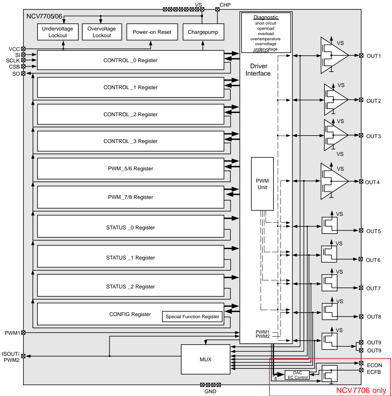
Figure 1. Block Diagram
