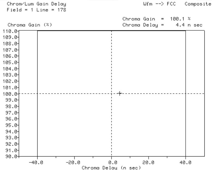
Figure 11. Chroma / Luma Gain & Delay
