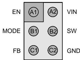
Figure 2. Top View
