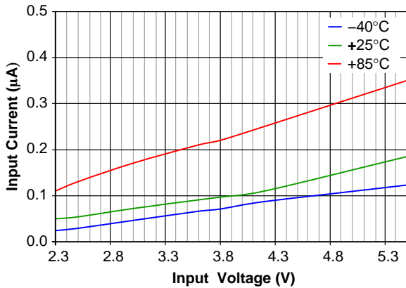
Figure 14. Shutdown Current vs. Input Voltage and Temperature
