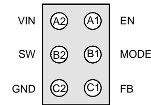
Figure 3. Bottom View
