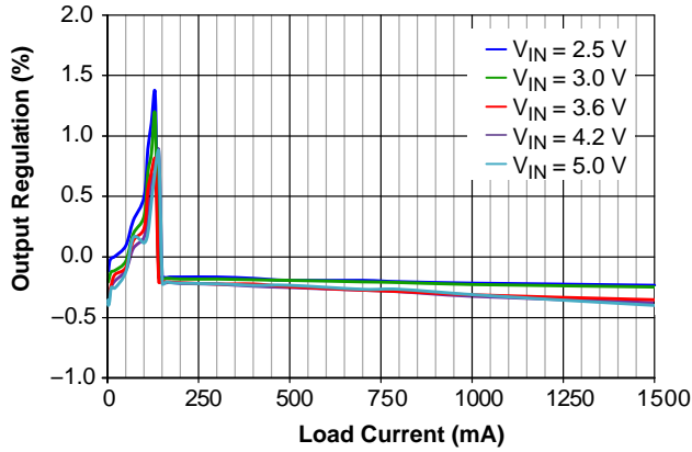
Figure 10. Output Regulation vs. Load Current and Input Voltage, V_{OUT} = 1.8\text{ V} , Auto Mode
