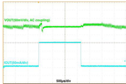
Figure 15. Load Transient, V_{IN} = 3.6\text{ V} , V_{OUT} = 1.8\text{ V} , 10\text{ mA} \leftrightarrow 150\text{ mA} , 1\text{ }\mu\text{s} Edge, Auto Mode
