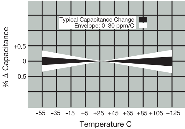
Temperature Coefficient
