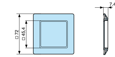
26546842 - Adaptor for 72 x 72 mm cut-out
