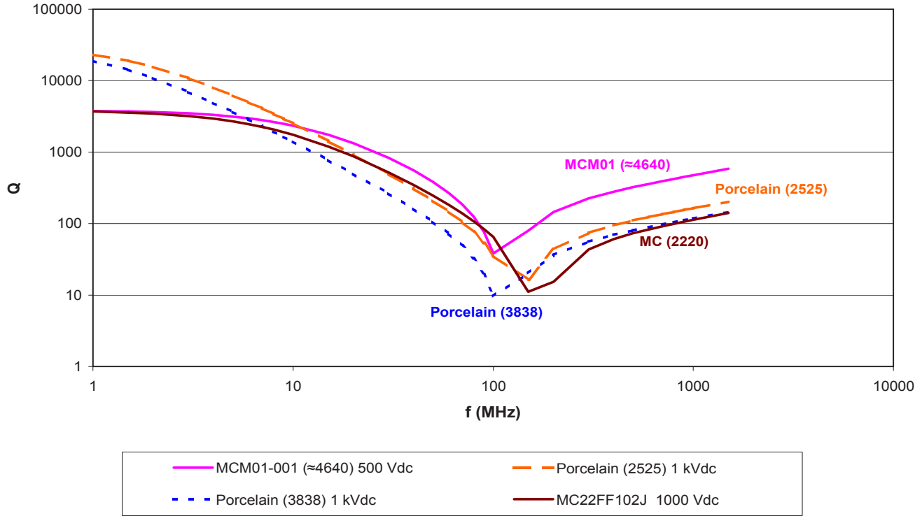
Q vs. Frequency for 1000 pF @ 25 °C
