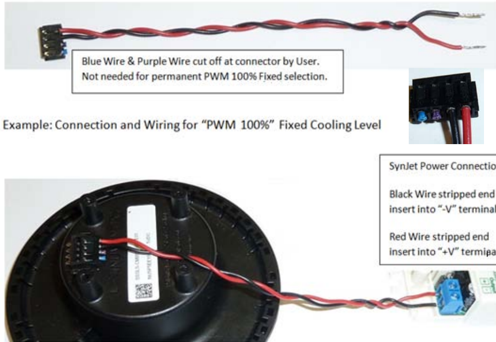
Figure 3. Permanent PWM 100% or CVC Maximum Cooling Level Selection
