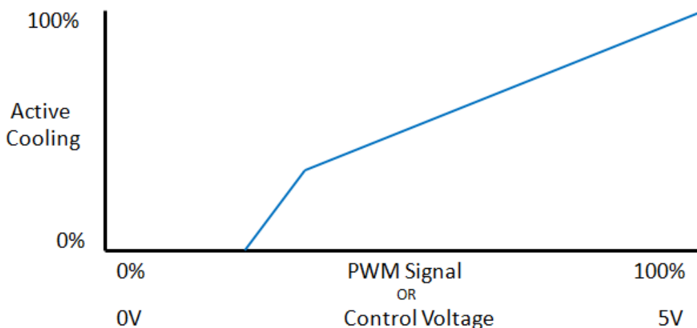
Figure 1. SynJet Active Cooling versus User Input Signal
