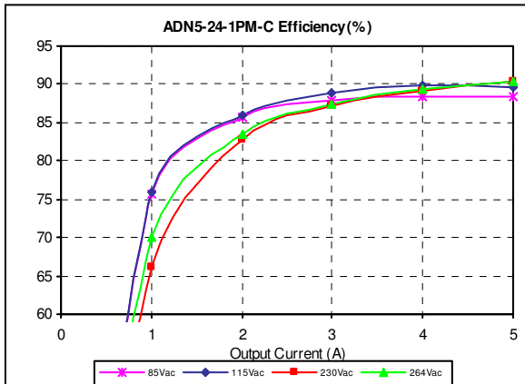
Figure 9: ADN5-24-1PM-C Efficiency Curves @ 25 °C, Convection Cool Vin = 85 to 264Vac Load: Io = 0 to 5.0A
