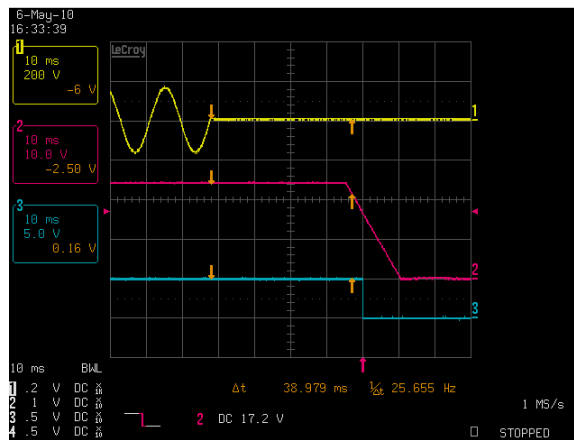
Figure 2: ADN5-24-1PM-C Hold-up Time (time to decay) Vin = 115Vac Load: Io = 5.0A Ch 1: AC Mains Ch 2: Vo Ch 3: DCOK
