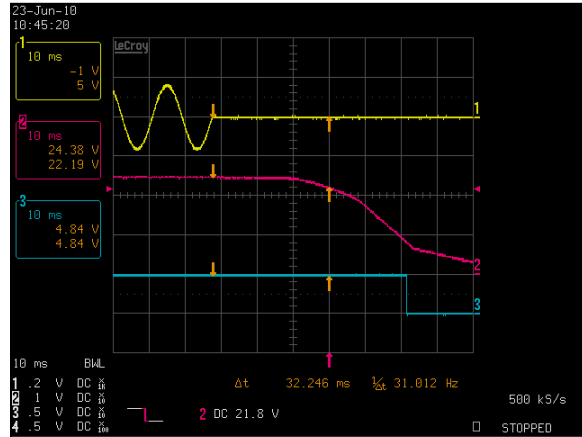
Figure 22: ADN20-24-1PM-C Hold-up Time (time to decay) Vin = 115Vac Load: Io = 20.0A Ch 1: AC Mains Ch 2: Vo Ch 3: DCOK
