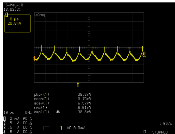
Figure 6: ADN5-24-1PM-C Ripple and Noise Measurement Vin = 115Vac Load: Io = 5.0A Ch 1: Vo
