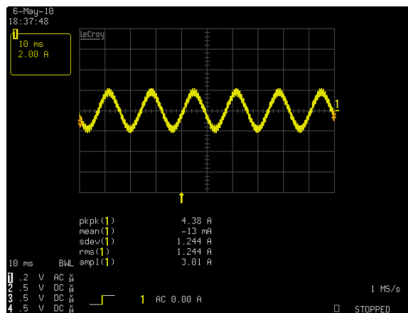
Figure 4: ADN5-24-1PM-C Input Current Waveform Vin = 115Vac Load: Io = 5.0A Ch 1: I N
