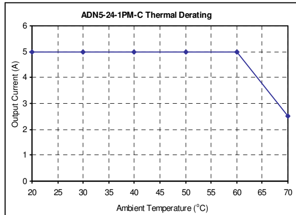
Figure 10: ADN5-24-1PM-C Derating Curves Vin = 115Vac Load: Io = 0 to 5.0A
