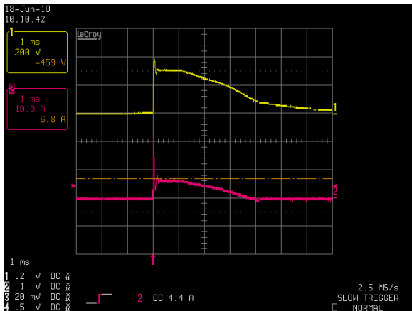
Figure 23: ADN20-24-1PM-C Inrush Current Vin = 230Vac Load: Io = 0A, Turn on angle = 90 deg Ch 1: AC Mains Ch 2: In
