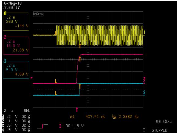
Figure 21: ADN20-24-1PM-C Turn-on delay Vin = 115Vac Load: Io = 20.0A Ch 1: AC Mains Ch 2: Vo Ch 3: DCOK
