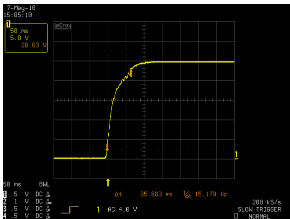
Figure 25: ADN20-24-1PM-C Output Voltage Startup Characteristic Vin = 90Vac Load: Io = 20.0A, Output Capacitance = 330uF/A Ch 1: Vo
