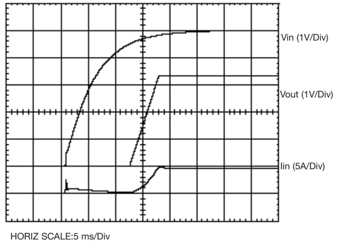
Figure 7 - Power-up Characteristic
