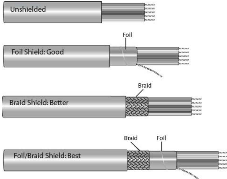
Figure 2. Typical shielding configurations
