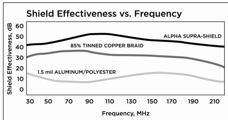
Figure 3. Foil-braid shielding yields the best shielding effectiveness
