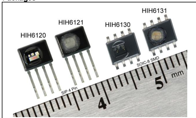
Figure 1. Honeywell HumidCon™ Digital Humidity/Temperature Sensors in SOIC-8 SMD and SIP 4 Pin Packages
