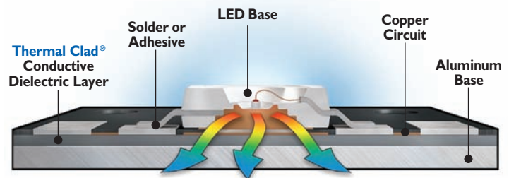
A Power LED's light output and life expectancy are directly attributed to how well the LED is managed thermally. As the LED generates heat, the dielectric of the Bergquist Thermal Clad metal core PCB quickly transfers it to the aluminum base, significantly improving the LED's performance.
