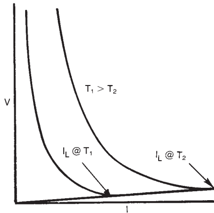
Figure 25: Voltage-Current Characteristic.
