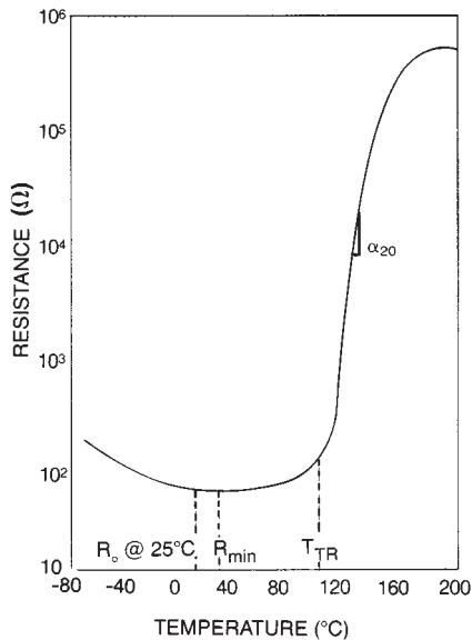
Figure 23: R-T Characteristic
